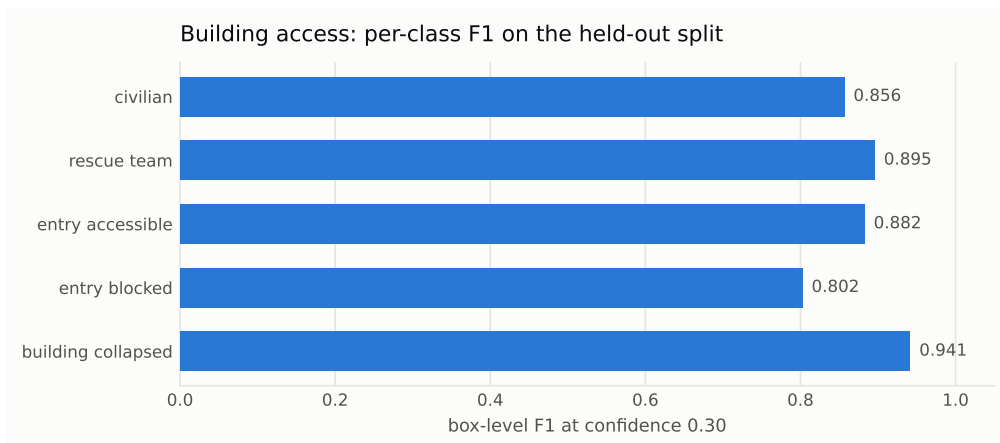
Figure 6. Per-class F_1 on the held-out split at confidence 0.30. Only civilian reaches the validator; the rest are operator context.
