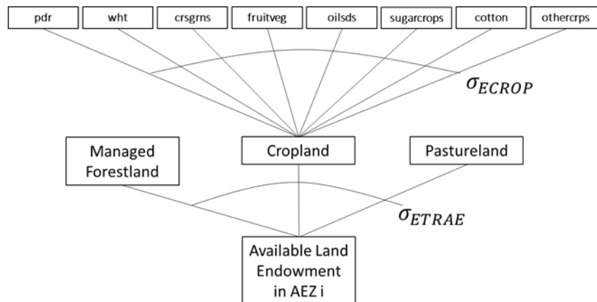
Figure S.2.3.2. Land supply in GTAP-AEZ
