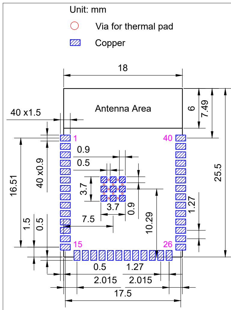
Figure 11-1. ESP32-S3-WROOM-1 Recommended PCB Land Pattern
