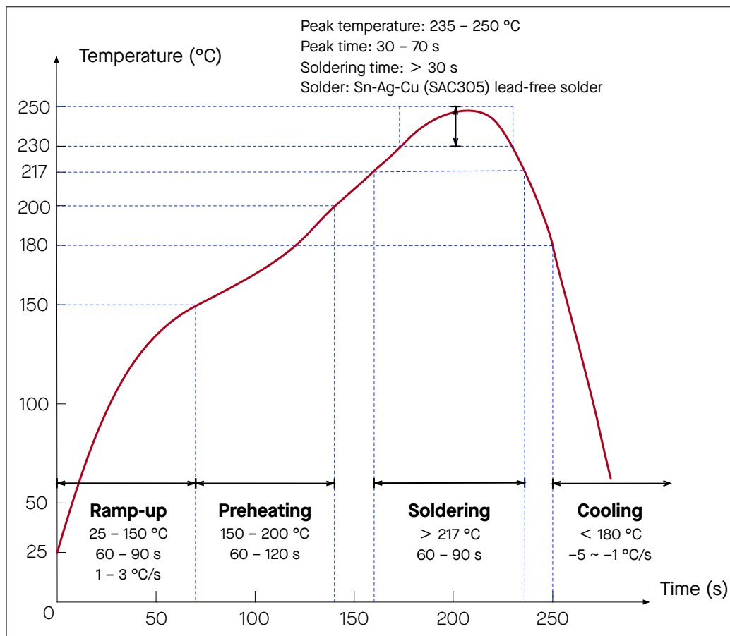
Figure 12-1. Reflow Profile
