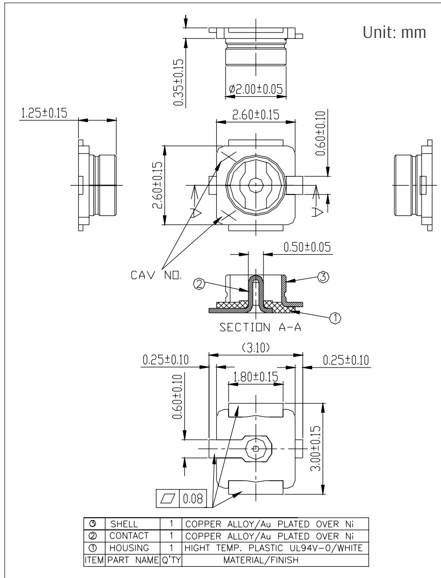
Figure 10-3. Dimensions of External Antenna Connector
