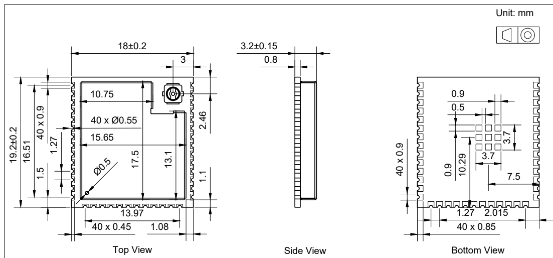
Figure 10-2. ESP32-S3-WROOM-1U Physical Dimensions
