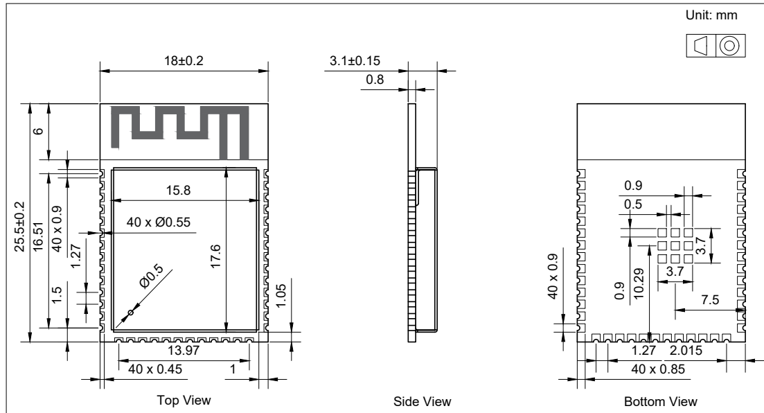
Figure 10-1. ESP32-S3-WROOM-1 Physical Dimensions
