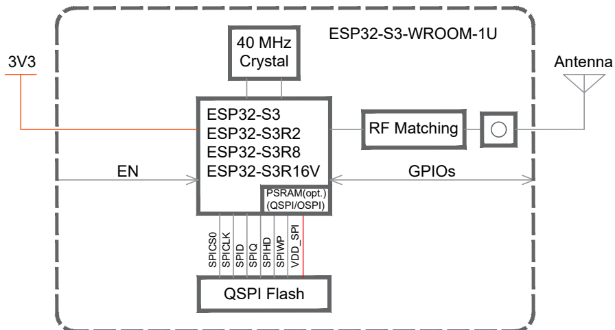
Figure 2-2. ESP32-S3-WROOM-1U Block Diagram
