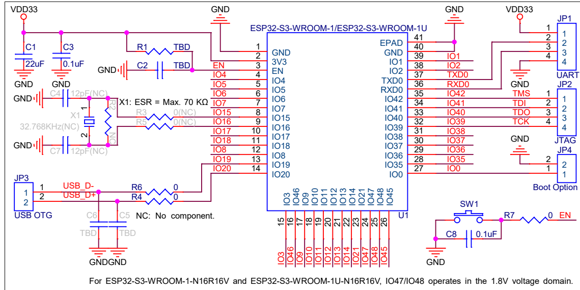
Figure 9-1. Peripheral Schematics
