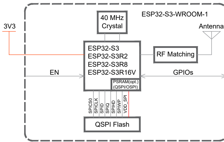
Figure 2-1. ESP32-S3-WROOM-1 Block Diagram
