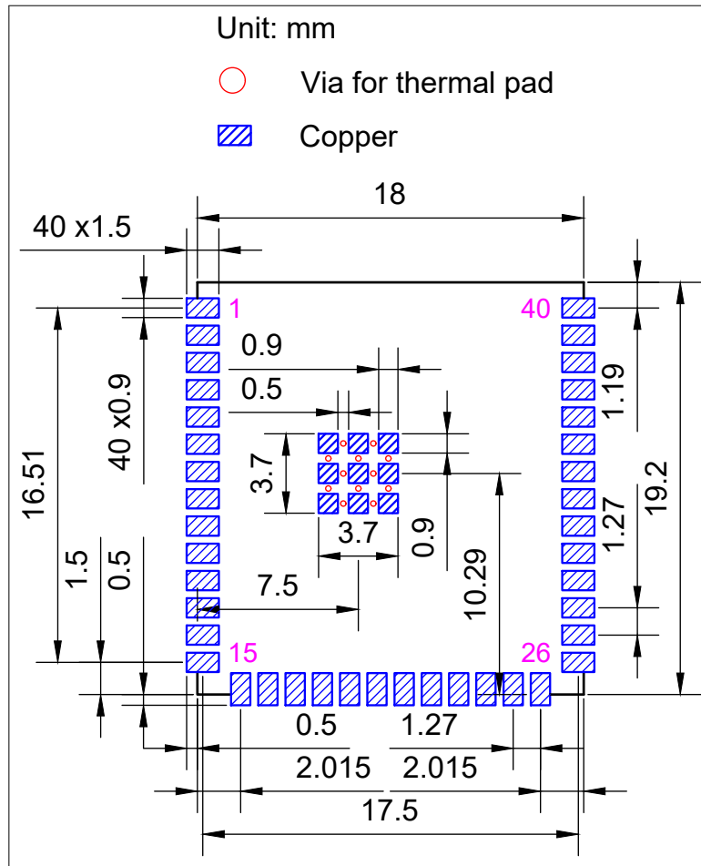
Figure 11-2. ESP32-S3-WROOM-1U Recommended PCB Land Pattern
