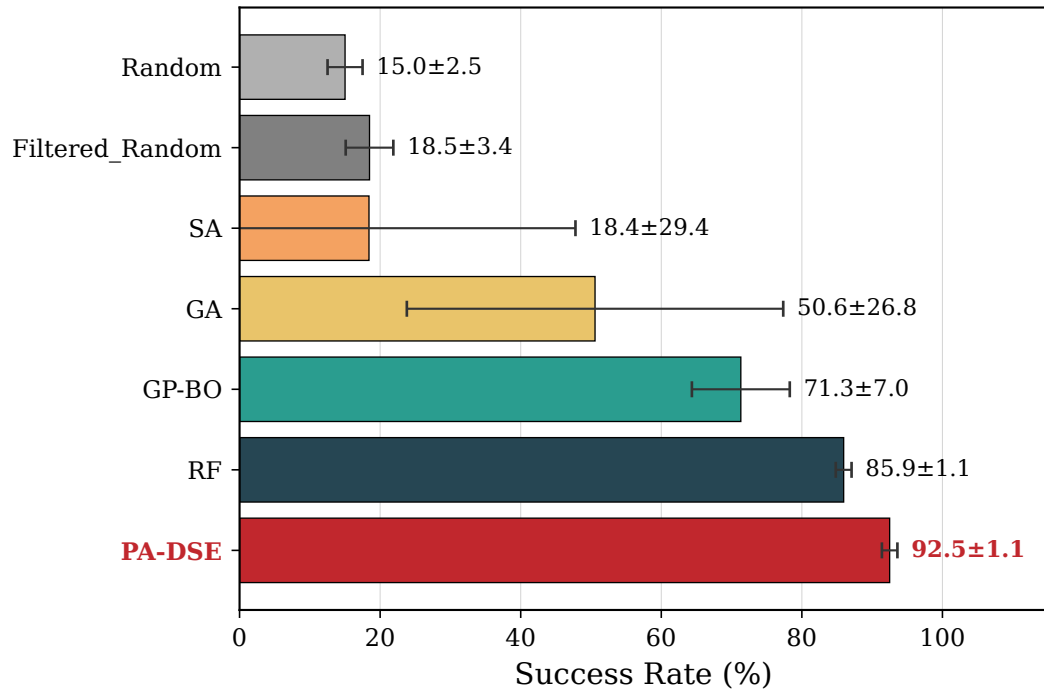
(a) Mean SR (across all runs)
