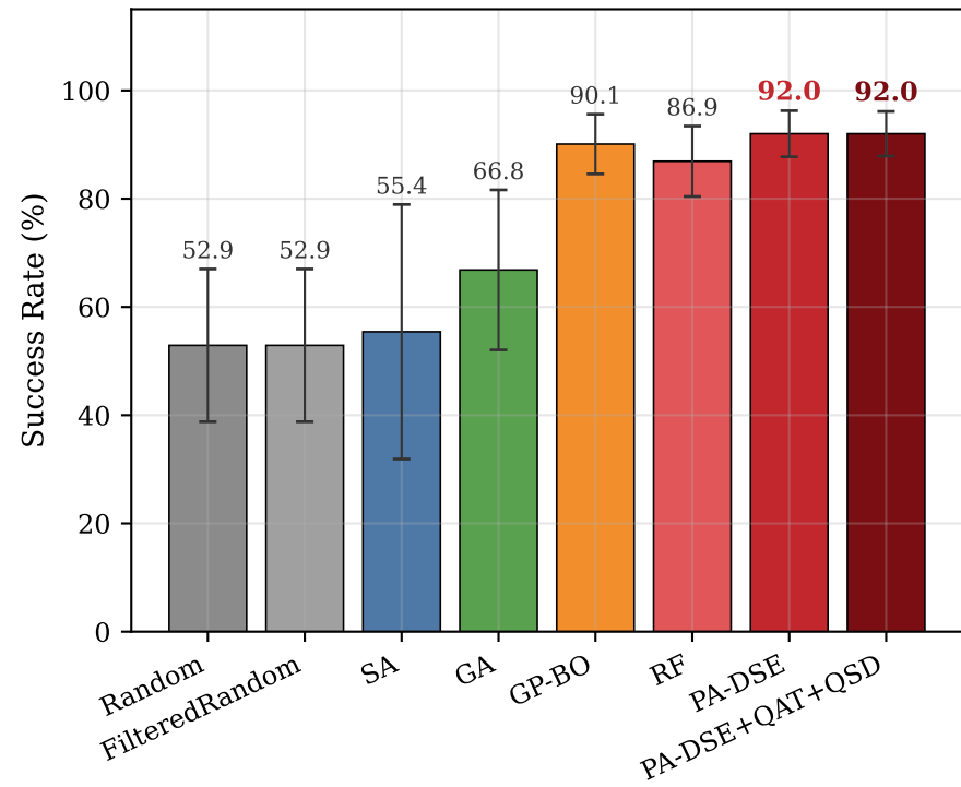
(a) Overall success rate (4 benchmarks)
