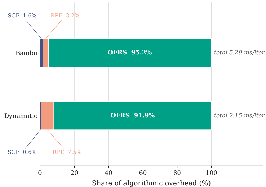
(b) Layer composition within algorithmic overhead
