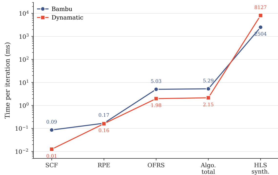
(a) Algorithmic overhead vs. HLS synthesis
