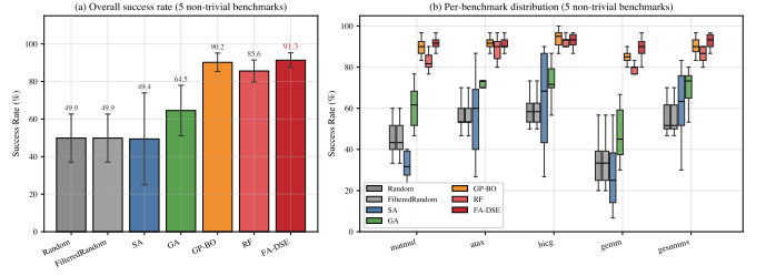
Fig. 3. Dynamatic main results ( B=30 ). (a) Aggregate SR with standard deviation across five non-trivial benchmarks. (b) Per-benchmark SR distribution. FA-DSE achieves the highest aggregate SR and remains competitive across non-trivial Dynamatic benchmarks, with lower variance among deployable methods.
