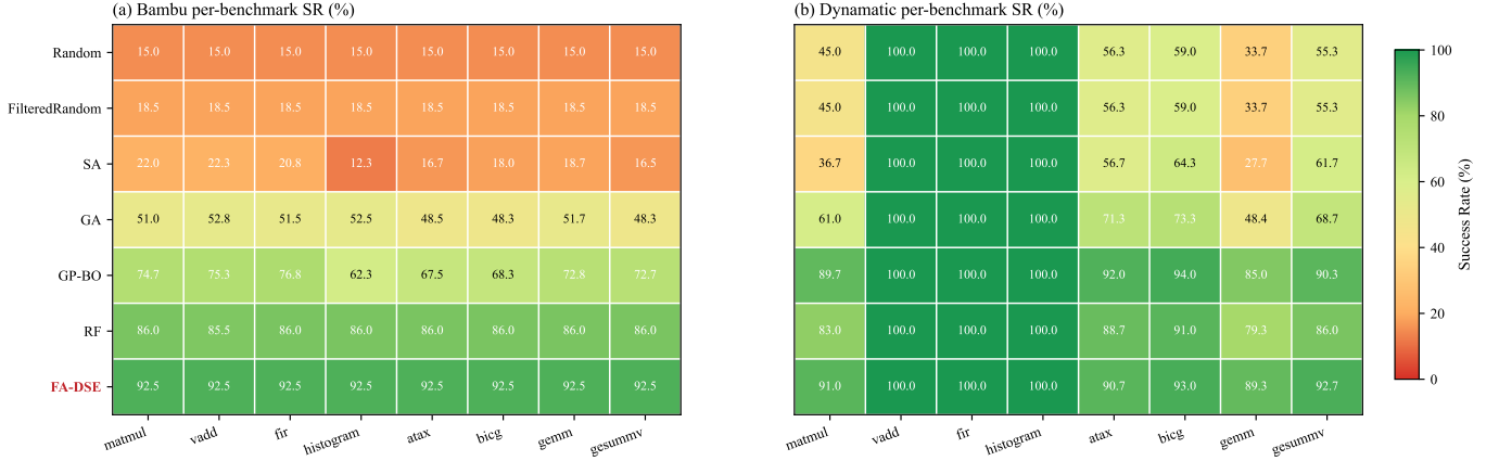
Fig. 5. Per-benchmark success rate (%). FA-DSE is consistently high across benchmarks: it wins or ties on all Bambu benchmarks and remains competitive on all Dynamic benchmarks, with low per-run variance. Several rows in panel (a) appear flat; this is structural, not an artifact (§V-D).
