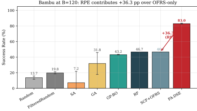
Fig. 9. Bambu at B=120 . RPE activates one signature per run, hard-skipping \sim 213 matching configurations and driving a +36.3pp SR gain over SCF+OFRS (which is identical to RF at this budget).
