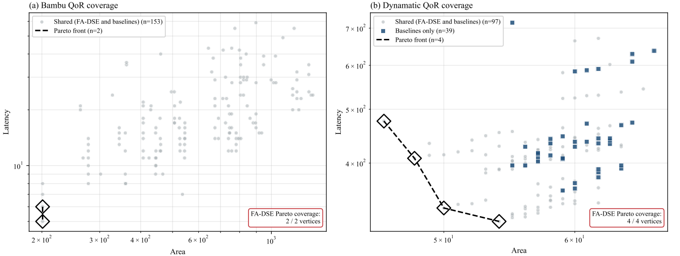
Fig. 7. QoR coverage comparison: each panel overlays the unique (area, latency) points discovered by FA-DSE and the union of baselines. Shared points (gray) are found by both; baseline-only points (blue) are missed by FA-DSE; Pareto-optimal vertices are marked with large diamonds. FA-DSE covers all Pareto-front vertices on both tools.
