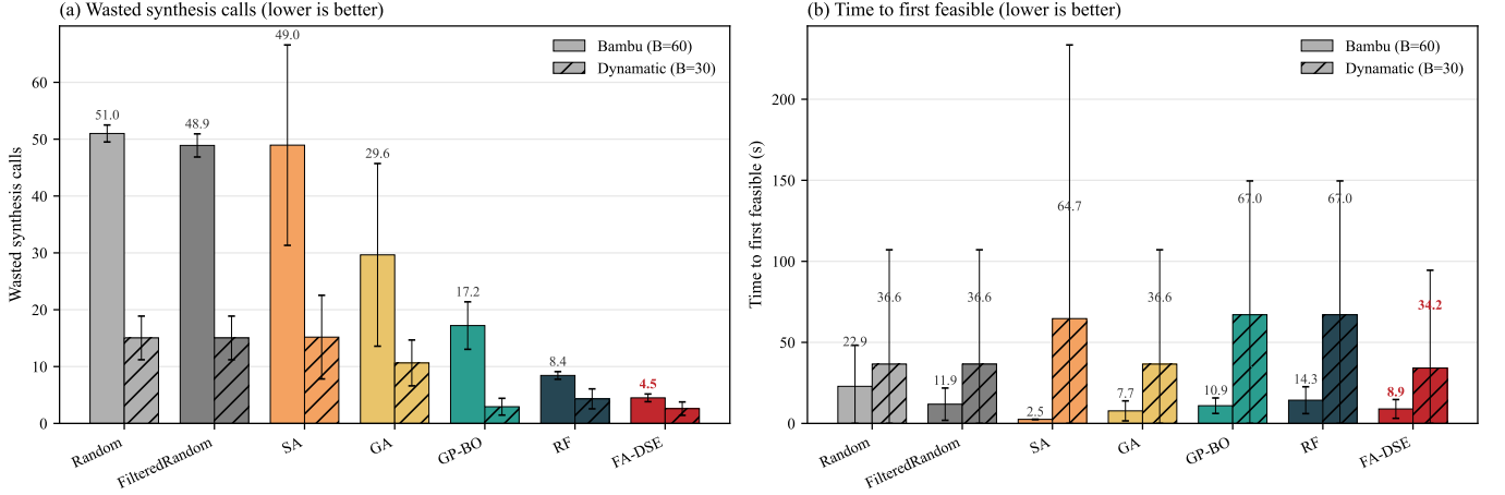
Fig. 4. User-visible cost. (a) Wasted synthesis calls per run (lower is better): FA-DSE wastes 4.5 on Bambu ( 1.9\times fewer than RF) and 2.6 on Dynamic (vs. 2.9 for GP-BO and 4.3 for RF). (b) Time to first feasible (lower is better): on Dynamic, FA-DSE reaches the first feasible design in half the wall-clock time of GP-BO and RF.
