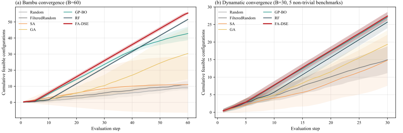
Fig. 6. Convergence curves (mean \pm 1\sigma across runs). (a) Bambu at B=60 : FA-DSE maintains near-linear progression throughout the budget, indicating that OFRS’s online reordering keeps promising configurations at the queue front. (b) Dynamic at B=30 : FA-DSE’s curve is steeper than the classical baselines, reflecting rapid learning of the dominant failure dimension.
