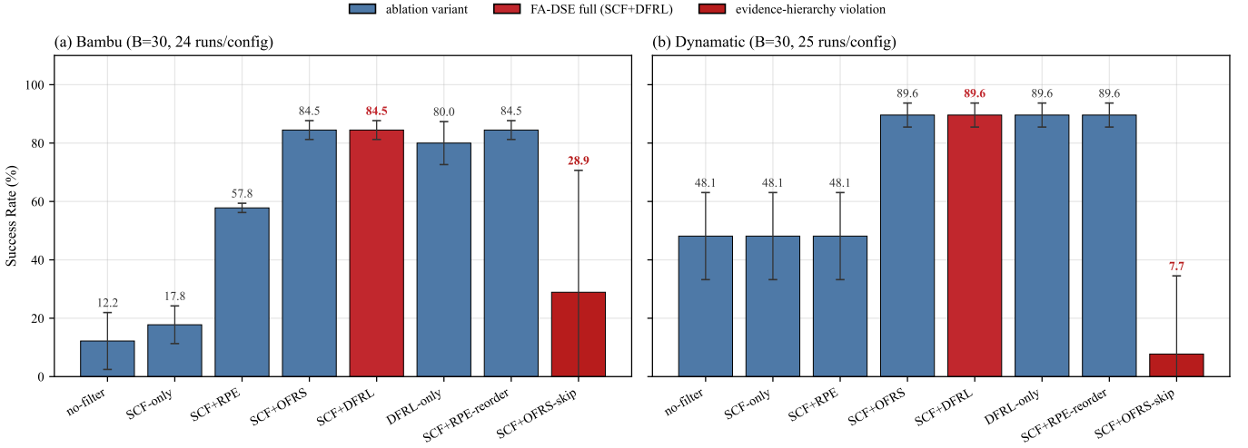
Fig. 8. Ablation study visualization ( B=30 ). FA-DSE full configuration (SCF+DFRL) highlighted in red. The rightmost bar (SCF+OFRS-skip, dark red) violates the evidence hierarchy by granting OFRS skip authority based on weak per-dimension evidence, producing order-of-magnitude larger variance and mean SR collapse on both tools.
