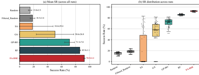
Fig. 2. Bambu main results ( B=60 ). (a) Mean SR with standard deviation error bars. (b) Per-run SR distribution: FA-DSE matches the tightest \sigma (1.1) among methods with non-trivial SR, while reaching the highest mean.
