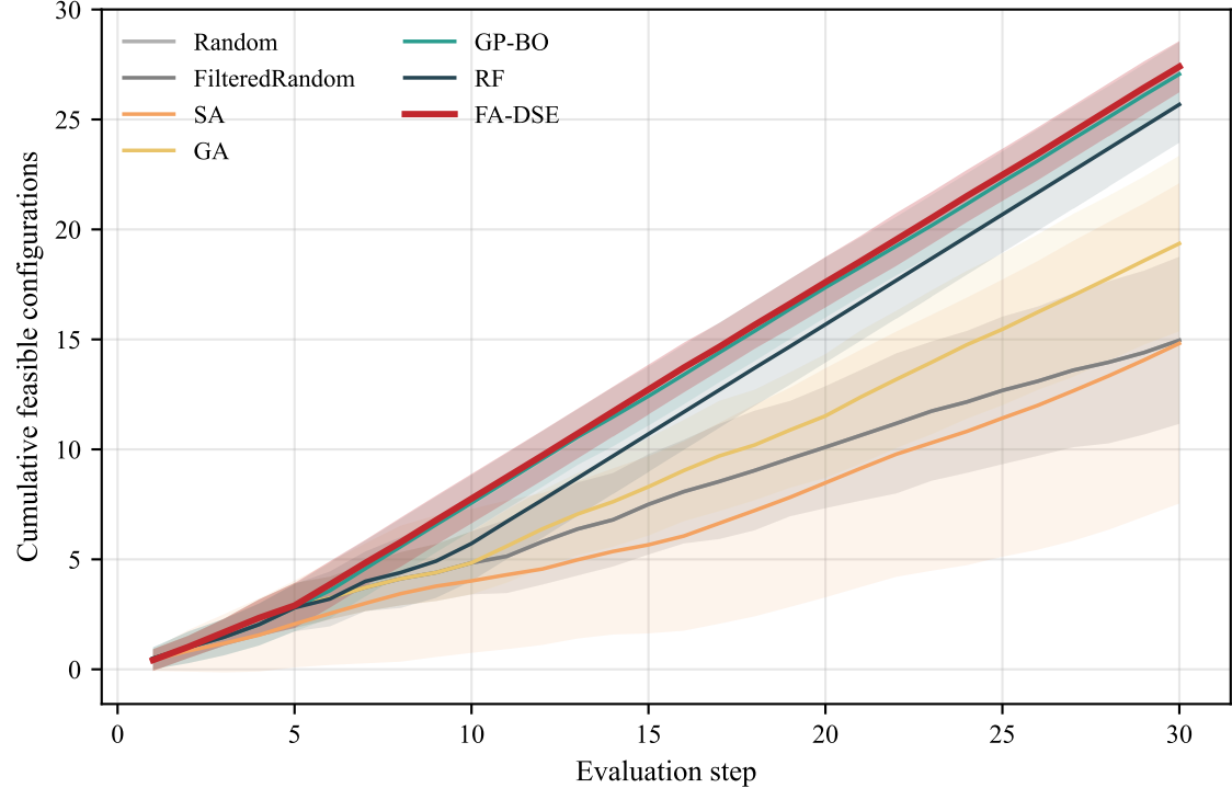
(b) Dynamic convergence (B=30, 5 non-trivial benchmarks)
