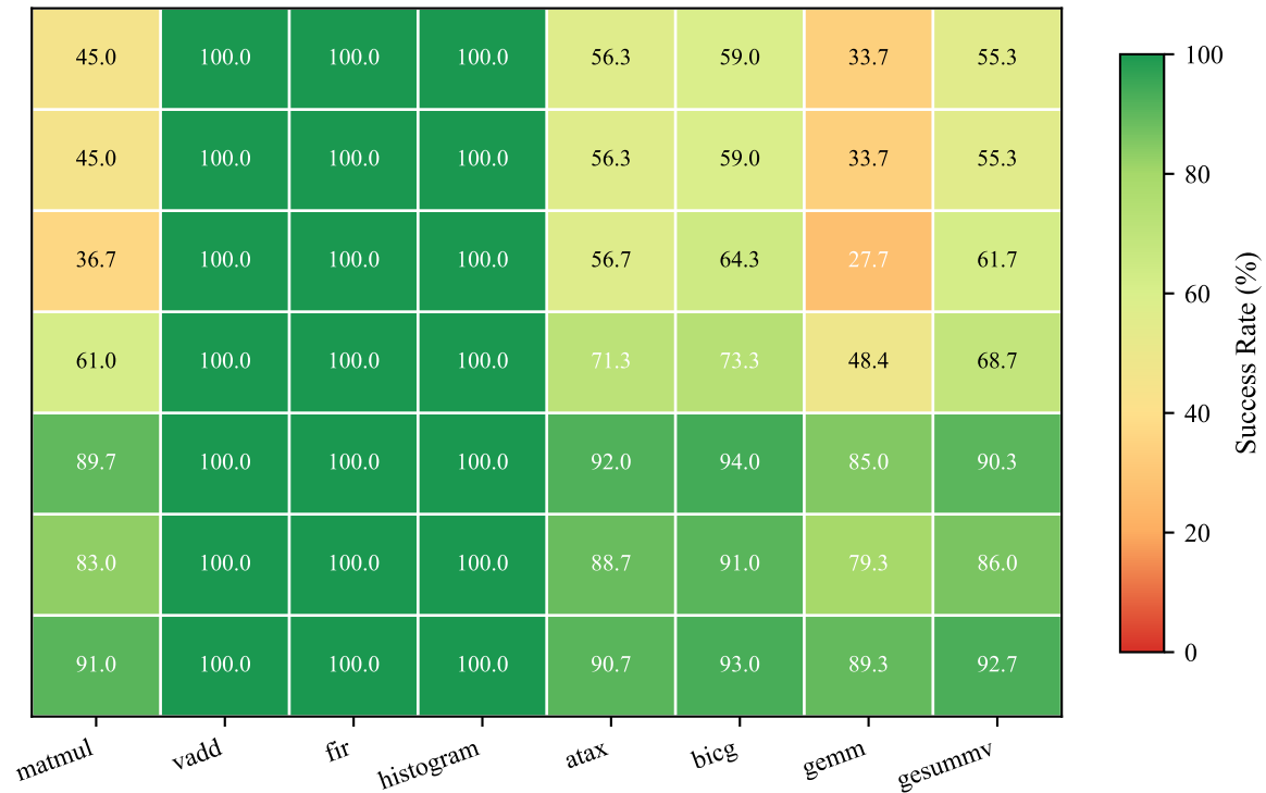
(b) Dynamatic per-benchmark SR (%)
