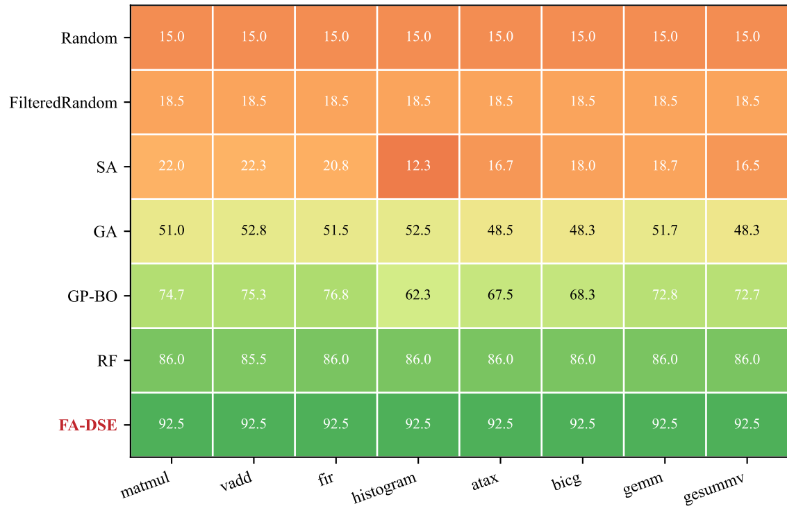
(a) Bambu per-benchmark SR (%)
