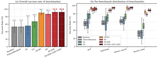
Fig. 3. Dynamic main results ( B=30 ). (a) Aggregate SR with standard deviation across four benchmarks. (b) Per-benchmark SR distribution. PA-DSE matches or exceeds all baselines across benchmarks with substantially lower variance.
