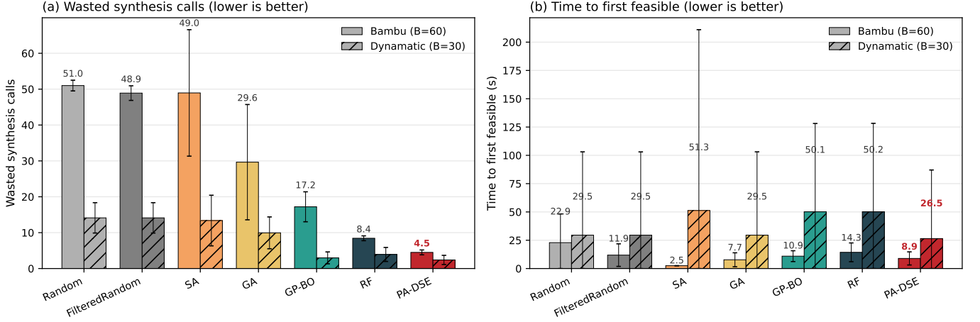
Fig. 4. User-visible cost. (a) Wasted synthesis calls per run (lower is better): PA-DSE wastes 4.5 on Bambu and 2.4 on Dynamic, a 1.9\times-11\times reduction over other methods. (b) Time to first feasible (lower is better): on Dynamic, PA-DSE reaches the first feasible design in half the wall-clock time of GP-BO and RF.
