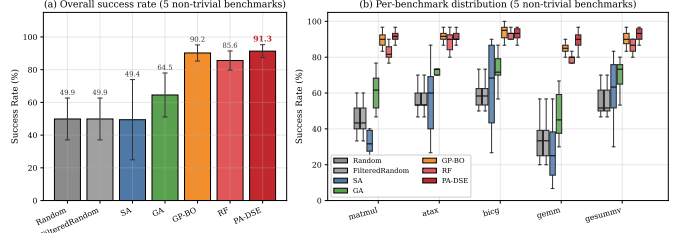
Fig. 3. Dynamatic main results ( B=30 ). (a) Aggregate SR with standard deviation across five non-trivial benchmarks. (b) Per-benchmark SR distribution. PA-DSE achieves the highest aggregate SR and remains competitive across non-trivial Dynamatic benchmarks, with lower variance among deployable methods.
