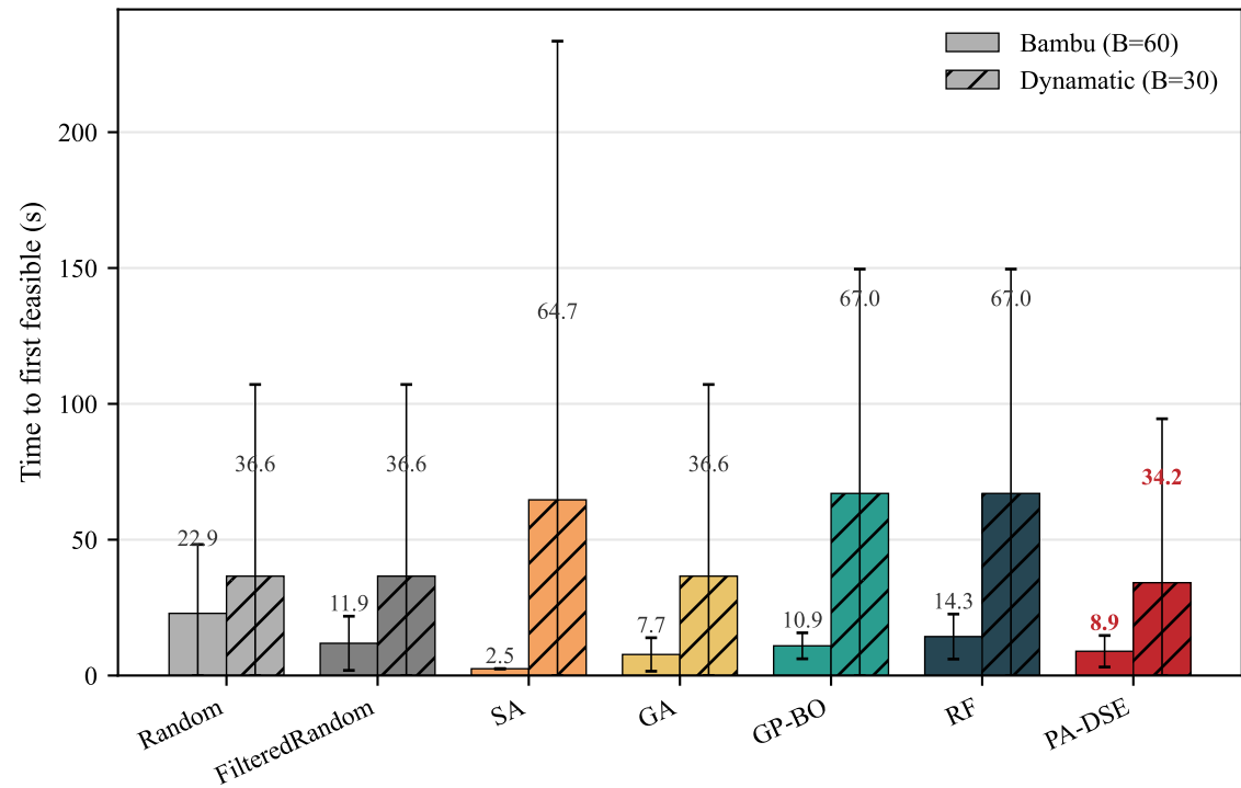
(b) Time to first feasible (lower is better)
