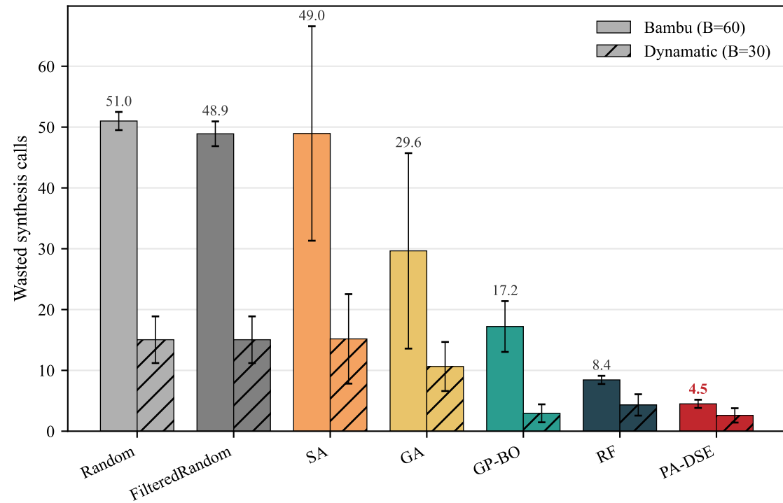
(a) Wasted synthesis calls (lower is better)
