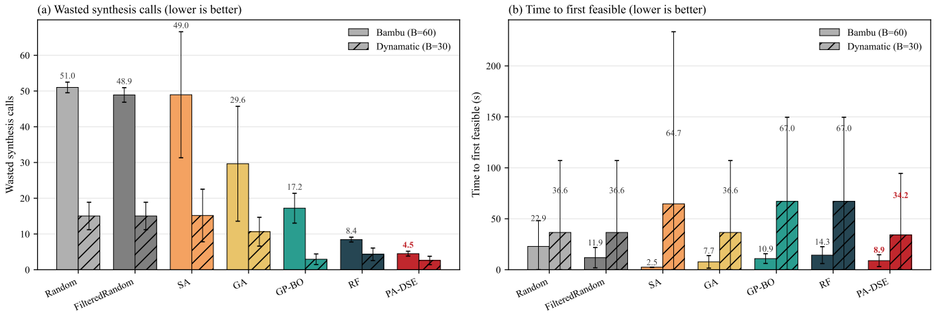
Fig. 4. User-visible cost. (a) Wasted synthesis calls per run (lower is better): PA-DSE wastes 4.5 on Bambu (1.9 \times fewer than RF) and 2.6 on Dynamatic (vs. 2.9 for GP-BO and 4.3 for RF). (b) Time to first feasible (lower is better): on Dynamatic, PA-DSE reaches the first feasible design in half the wall-clock time of GP-BO and RF.
