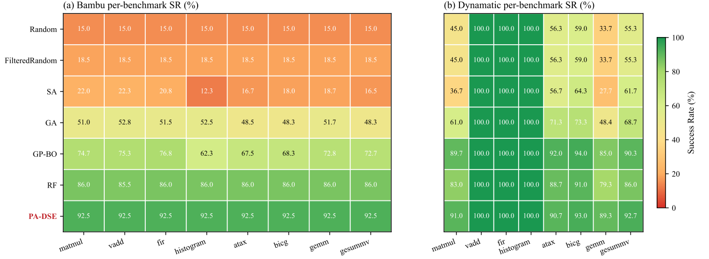
Fig. 5. Per-benchmark success rate (%). PA-DSE wins or ties on every benchmark with the tightest per-run variance. Several rows in panel (a) appear flat; this is structural, not an artifact (§V-D).
