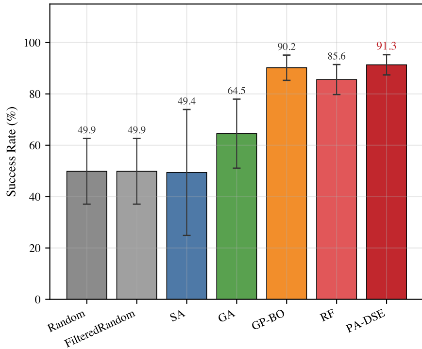
(a) Overall success rate (5 non-trivial benchmarks)
