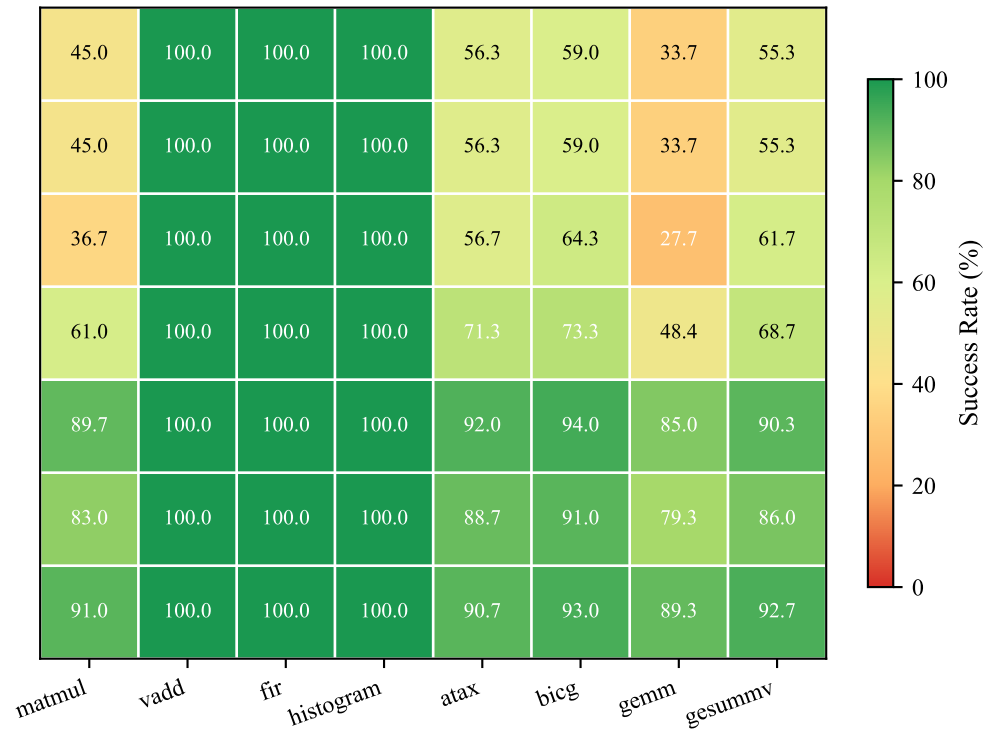
(b) Dynamatic per-benchmark SR (%)
