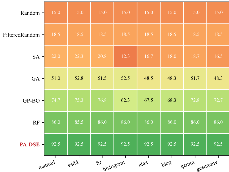
(a) Bambu per-benchmark SR (%)
