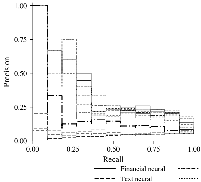
(a) Precision–recall
