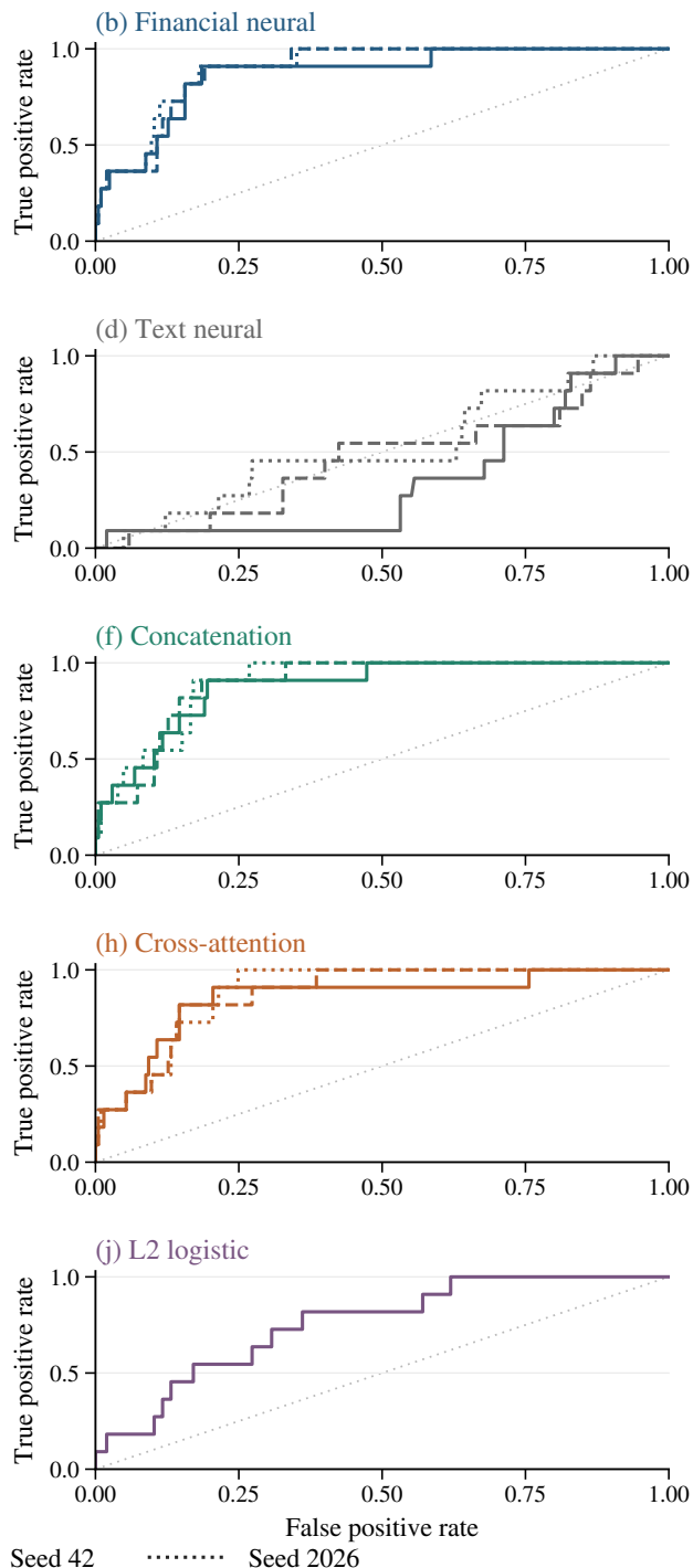
Receiver operating characteristic
