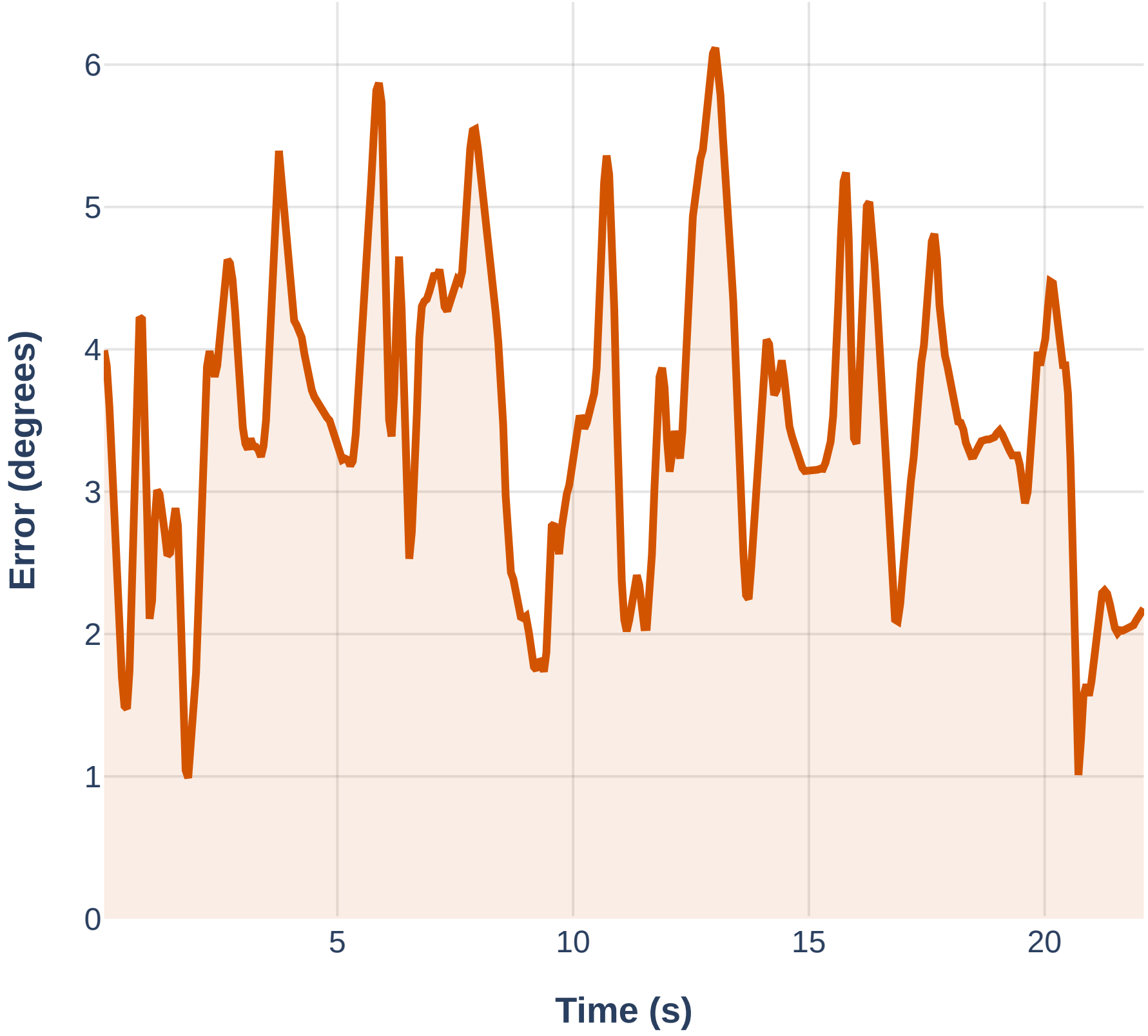
Orientation Error
