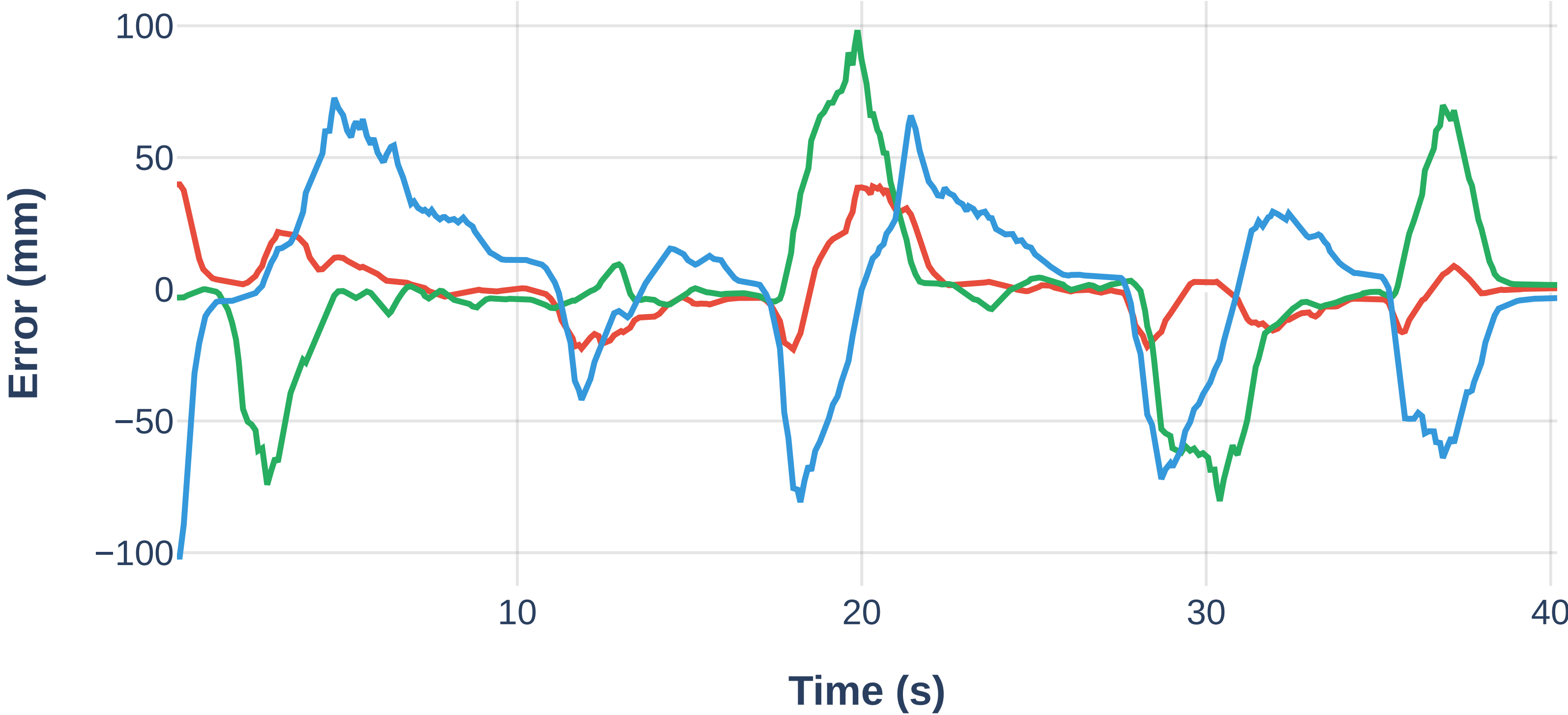
Position Error Components
