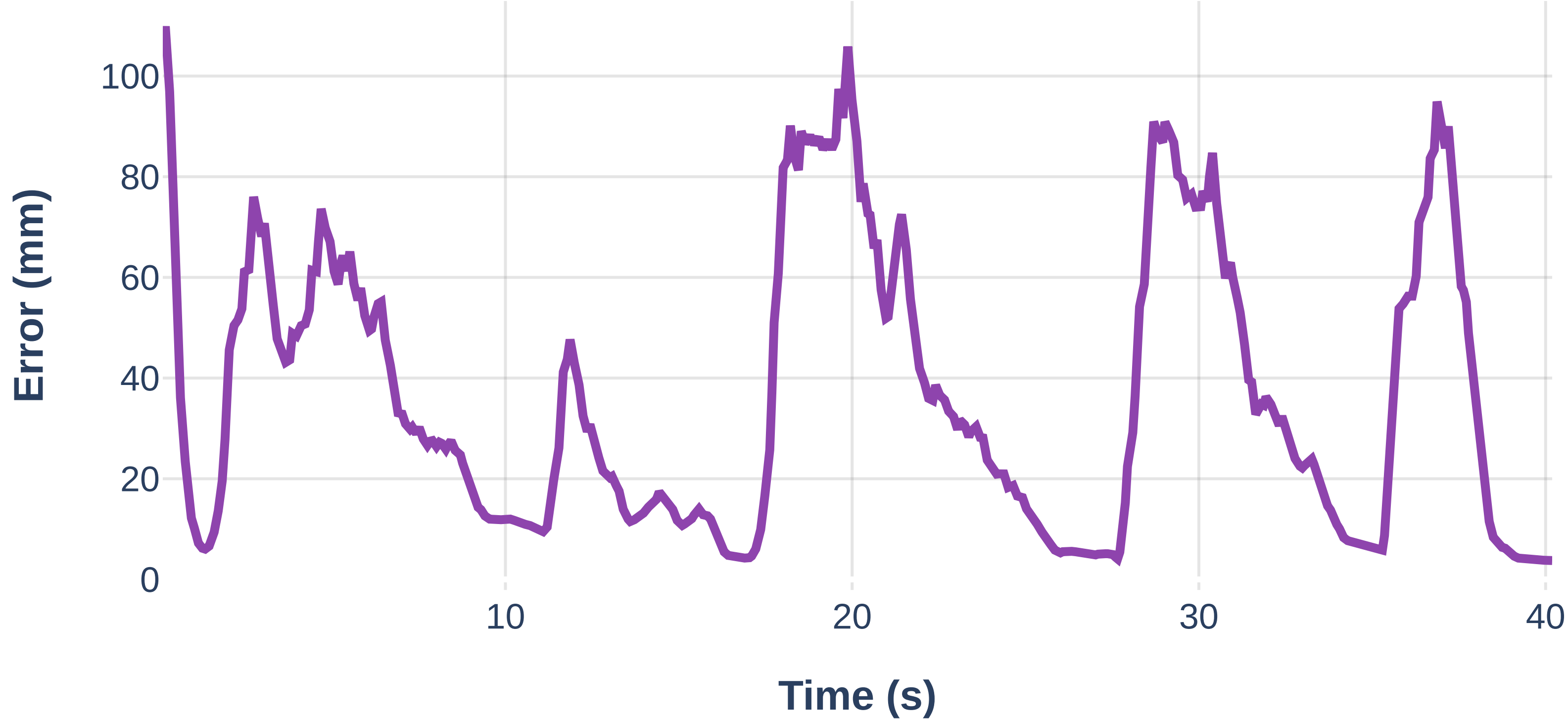
Position Error vs Time
