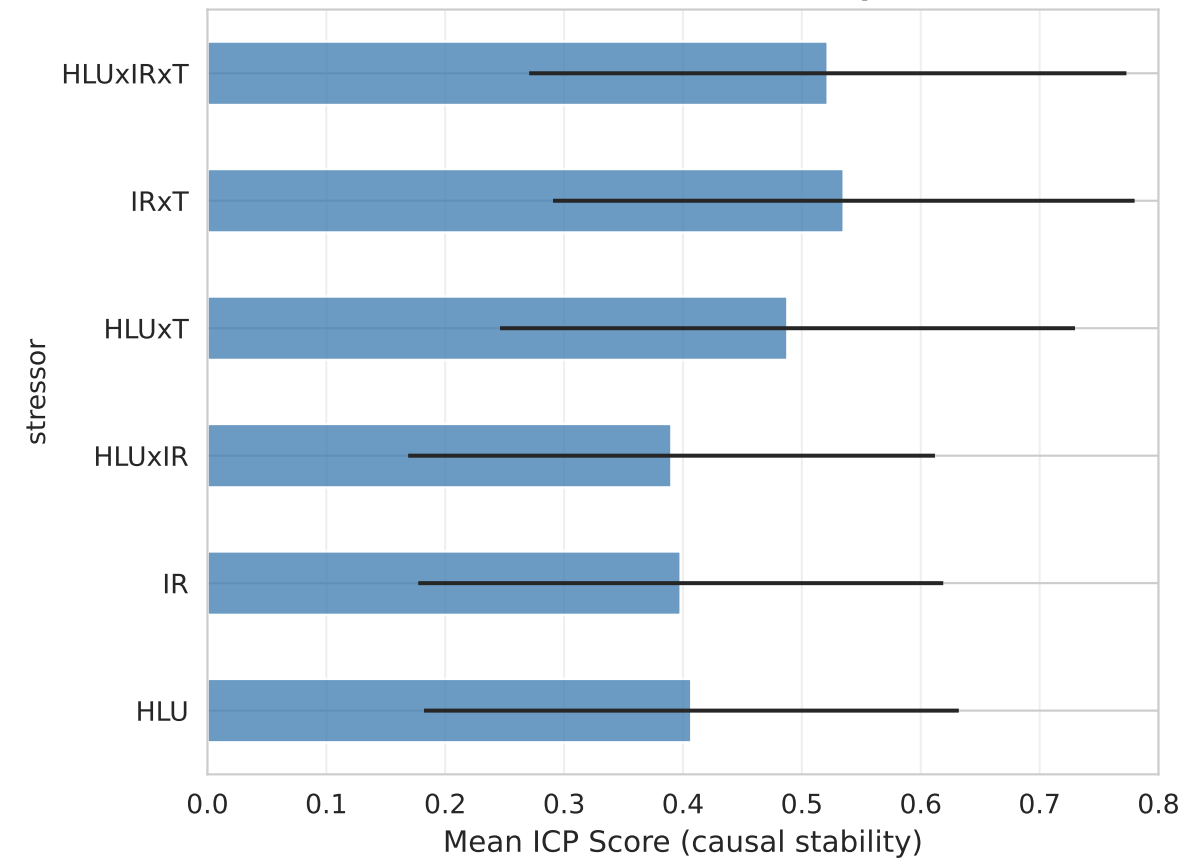
B. Stressor Causal Stability (ICP)
