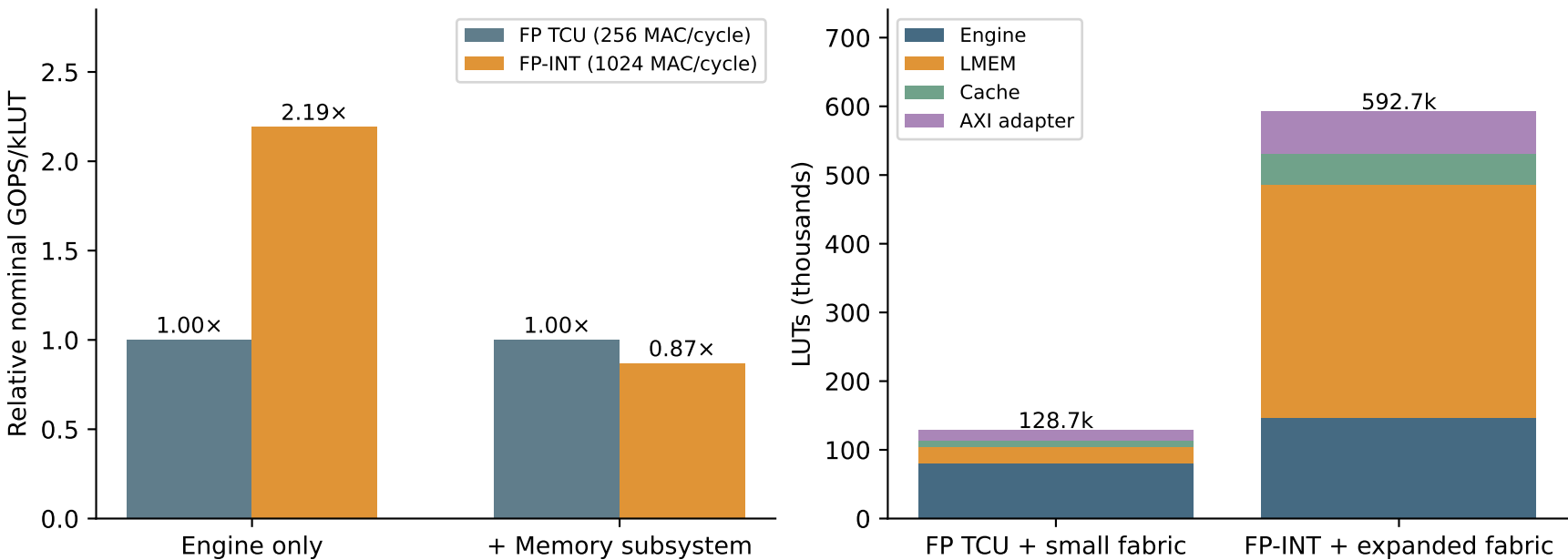
Fig. 5 FPGA draft: separately synthesized block costs OOC synthesis + opt_design; nominal throughput at 100 MHz, no routing
