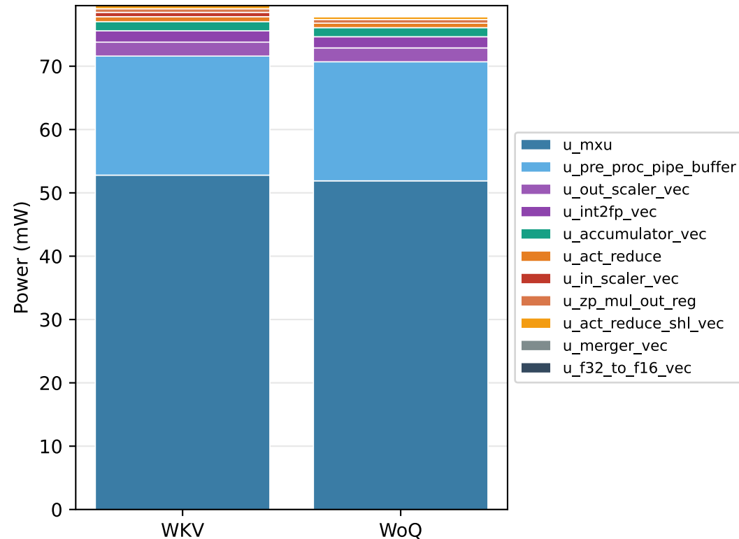
Module-level power
