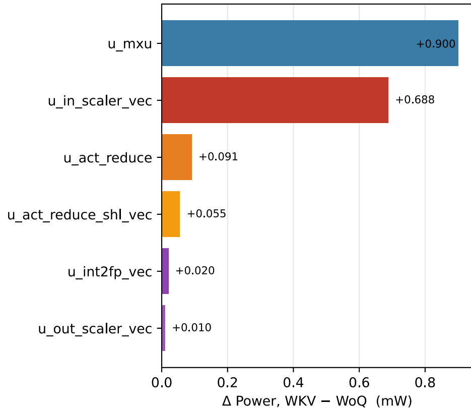
WKV overhead per block — total 1.76 mW
