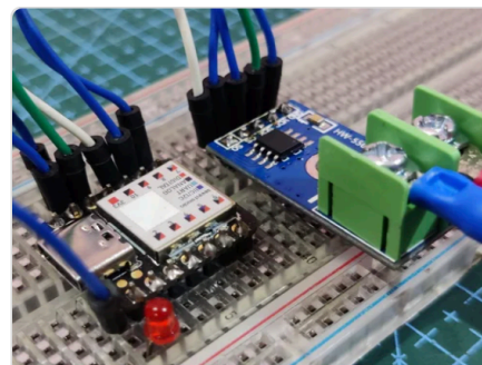
MAX6675 Temp Sensor With XIAO M0
