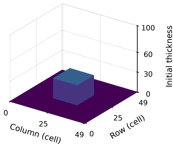
(c) Center-30
