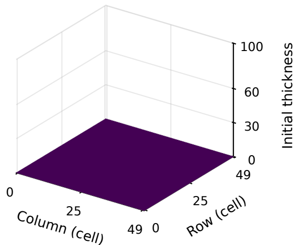
(c) Center-30
