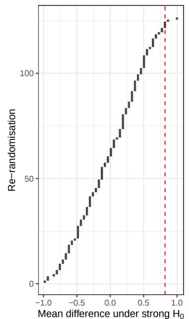
Figure 4.3: There are 126 different ways in which the 9 participants could have been split up into two groups so that there are five participants in the experimental group. These are the differences between the means for all 126 possibilities under the strong null hypothesis. The mean difference we actually observed (0.82) is represented by the dashed red vertical line.
