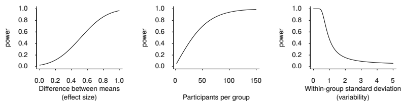
Figure 4.5: These three graphs show how the statistical power of a study varies with the effect size (left), the number of observations per group (middle) and the variability in the outcome variable within each group (right).
