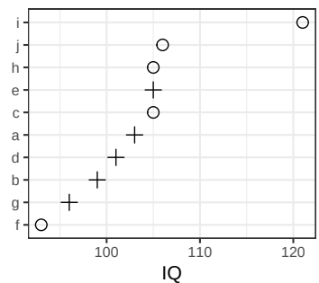
Figure 2.2: Ten participants sign up for a study. You measure their IQ and you also know their sex (represented here by circles and pluses). Figure 2.3: Six possible random assignments (out of 252) of the ten participants from Figure 2.2. The dotted vertical lines show the mean IQ in each group.
