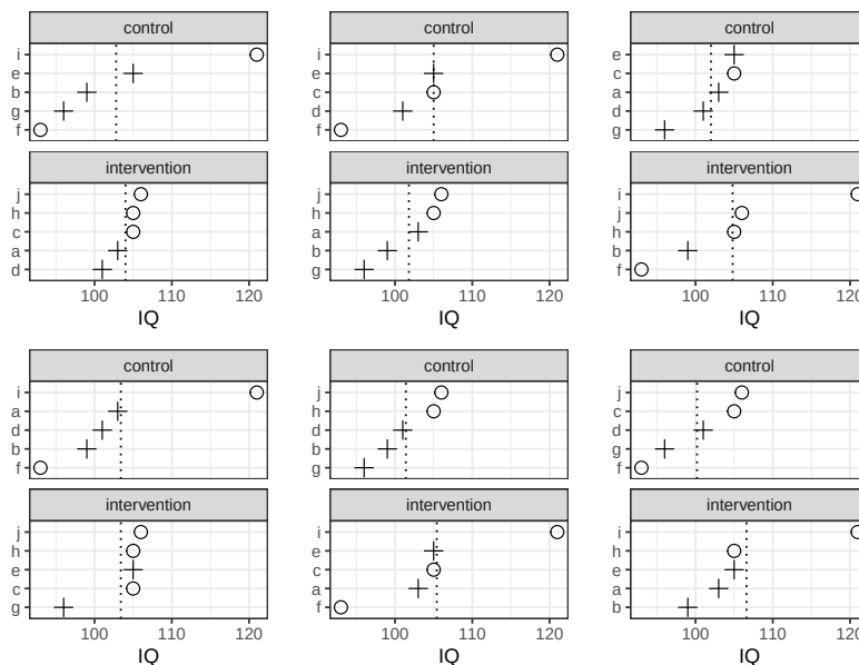
Figure 2.2: Ten participants sign up for a study. You measure their IQ and you also know their sex (represented here by circles and pluses). Figure 2.3: Six possible random assignments (out of 252) of the ten participants from Figure 2.2. The dotted vertical lines show the mean IQ in each group.
