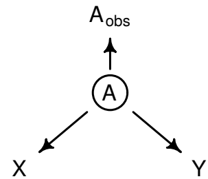
Figure 9.1: The X - Y relationship is confounded by A . A , however, can't be observed directly. A proxy (indicator) A_{\text{obs}} can be controlled for instead, but this won't fully shut the non-causal path X \leftarrow A \rightarrow Y .
