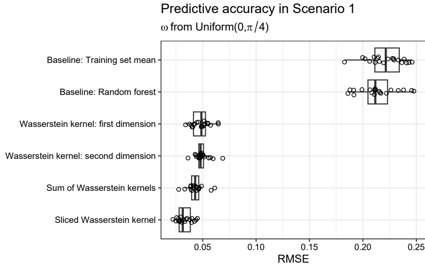
Figure 4.2: The root mean squared errors obtained by each prediction model for the twenty runs of the toy example in the first scenario (rotation angle drawn from Uniform( 0, \pi/4 )).
