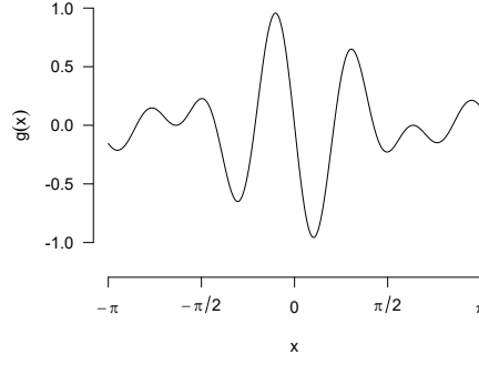
Figure 5.2: The function g used to generate the outcome data.
