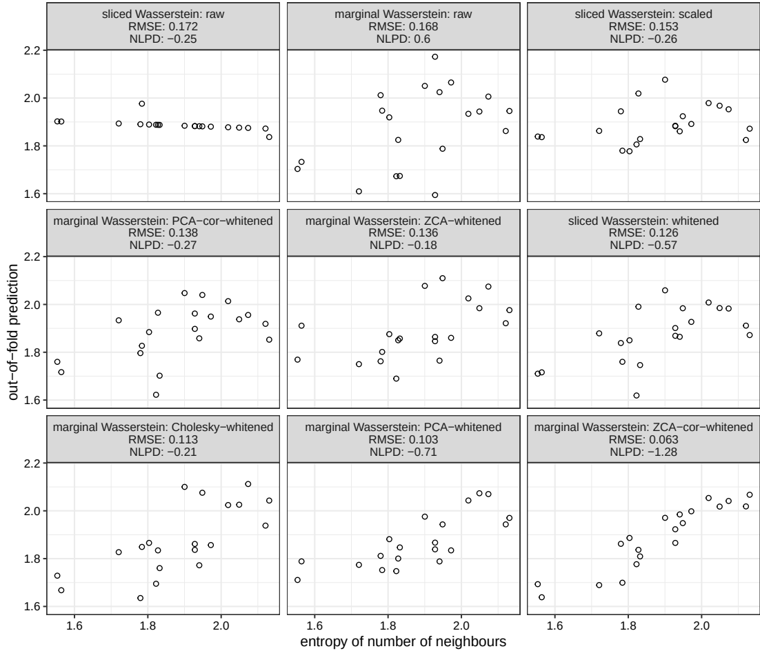
Figure 5.6: Out-of-fold predictions for the entropy of the empirical distributions of the number of neighbours by nine models based on different kernels. The facets are sorted left to right, top to bottom, in order of descending root mean squared error (RMSE). The root mean squared error of a baseline model that uses the mean of the in-fold outcomes as the prediction was 0.165, meaning that both the sliced and marginal Wasserstein kernels based on the raw input matrices could not beat this baseline. The average negative log predictive density (NLPD) scores are reported as well.
