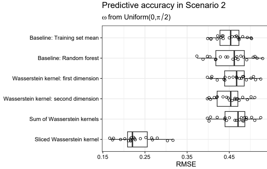
Figure 4.3: The root mean squared errors obtained by each prediction model for the twenty runs of the toy example in the second scenario (rotation angles drawn from Uniform( 0, \pi/2 )).
