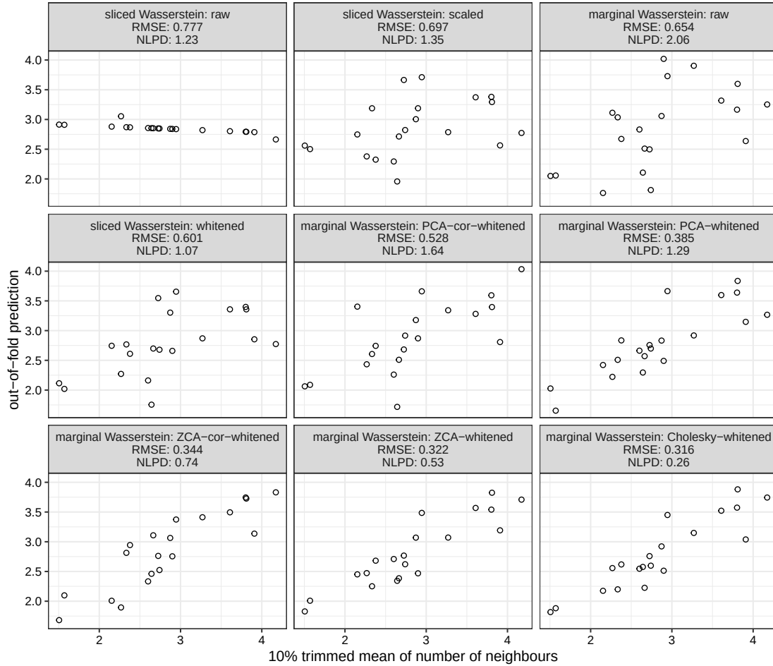
Figure 5.5: Out-of-fold predictions for 10% trimmed means of the number of neighbours by nine models based on different kernels. The facets are sorted left to right, top to bottom, in order of descending root mean squared error (RMSE). The root mean squared error of a baseline model that uses the mean of the in-fold outcomes as the prediction was 0.759, meaning that sliced Wasserstein kernel based on the raw input matrices could not beat this baseline. The average negative log predictive density (NLPD) scores are reported as well.
