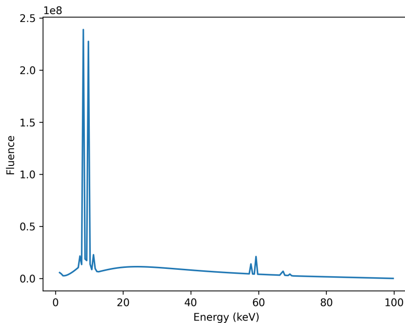
FIGURE 10.4: X-ray spectrum for a tungsten cathode at 100 kVp showing the continuous bremsstrahlung spectrum and characteristic peaks. Build with SpekPy [17]
