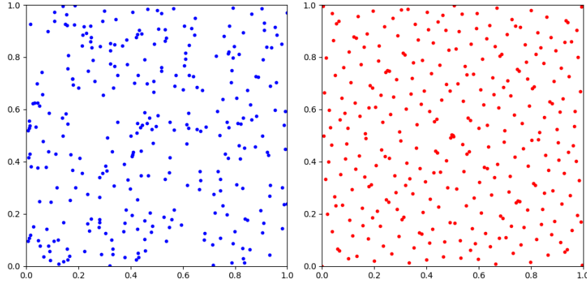
FIGURE 1.1: Comparison of 300 randomly drawn sample points in [0, 1]^2 using standard MC (left) and the first 300 elements of the Sobol' sequence in 2 dimension.
