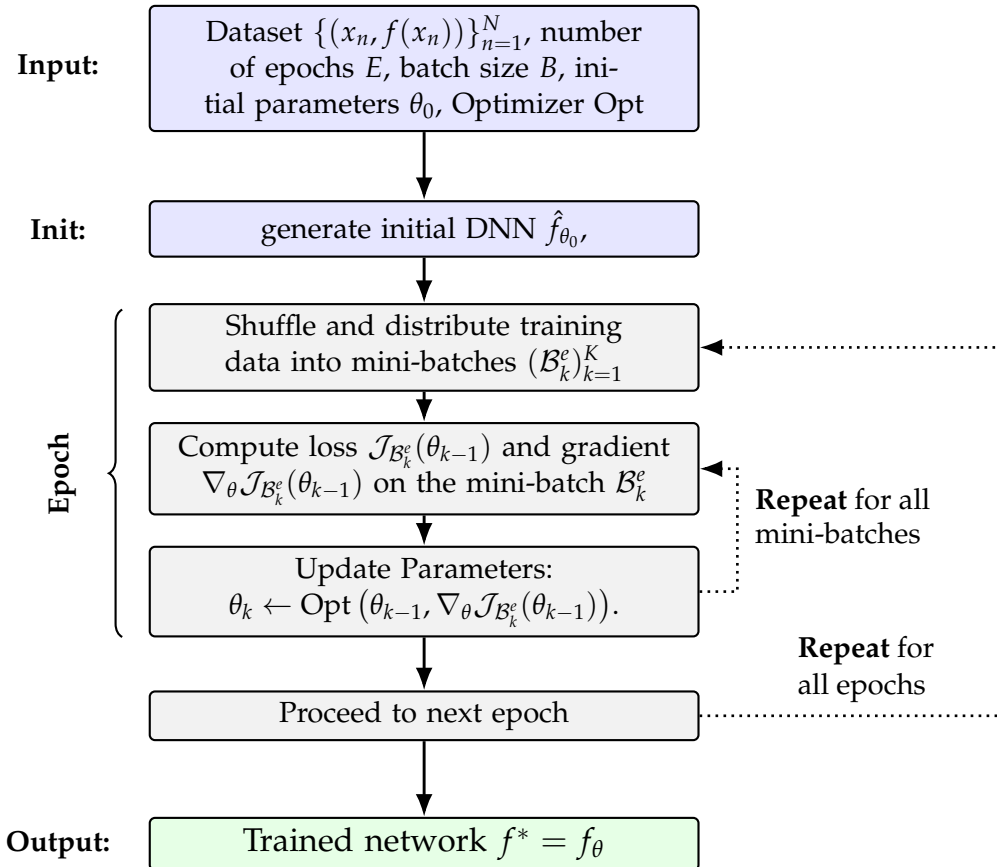
FIGURE 5.3: Generic DNN training: for each of E epochs, iterate over mini-batches of size B , compute loss/gradients and update parameters using optimizer Opt.
