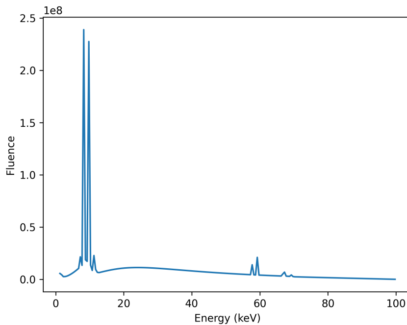
FIGURE 9.4: X-ray spectrum for a tungsten cathode at 100 kVp showing the continuous bremsstrahlung spectrum and characteristic peaks. Build with SpekPy [18]
