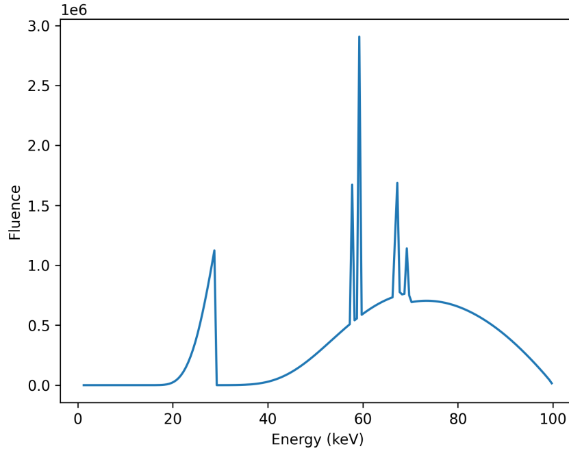
FIGURE 9.6: X-ray spectrum for a tungsten cathode at 100 kVp with a 0.4 mm showing the continuous bremsstrahlung spectrum and characteristic peaks. Build with SpekPy [18]
