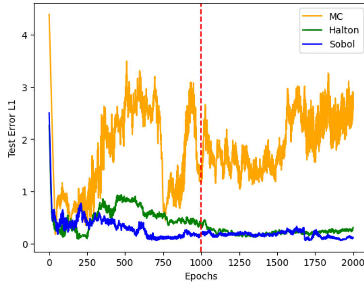
FIGURE 7.1: Test error for training set size N = 4096 for the 6D sum of sines function.
