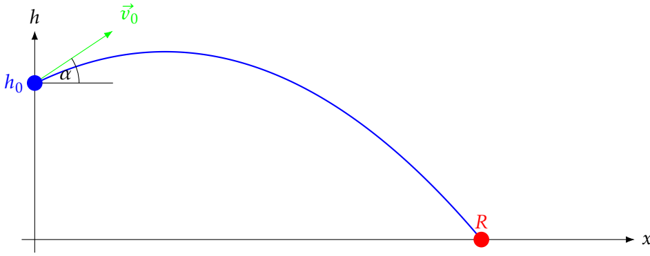
FIGURE 7.3: Projectile motion setup with projectile launched from height h_0 and initial velocity \vec{v}_0 at angle \alpha to the horizontal. The final range R is achieved at impact time t_\star .
