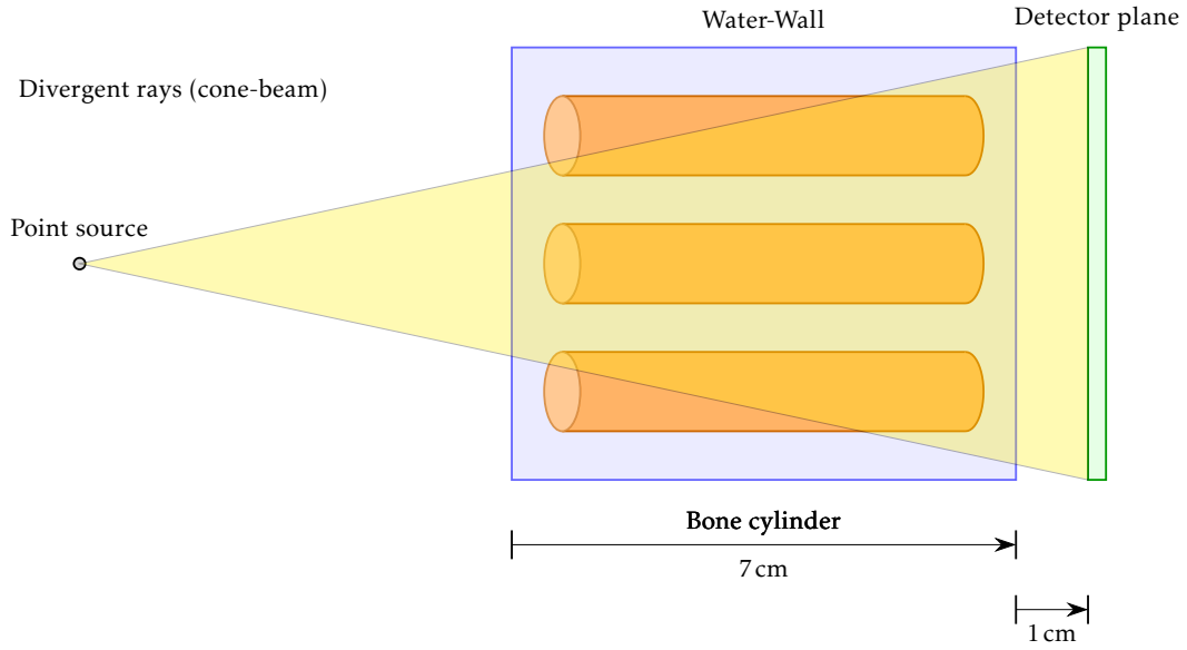
FIGURE 11.2: Point source emitting cone-beam rays through a water-wall containing bone cylinders.
