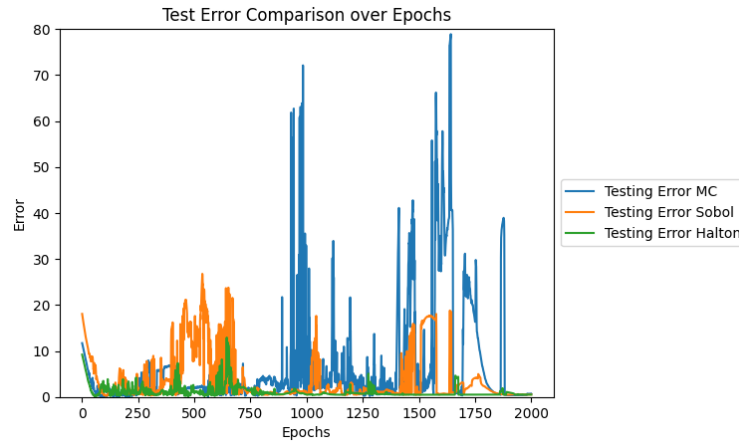
FIGURE 7.2: Test error for the 8D sum of sines function (7.1) for different sizes N and different training set sampling strategies using Adam as optimizer.
