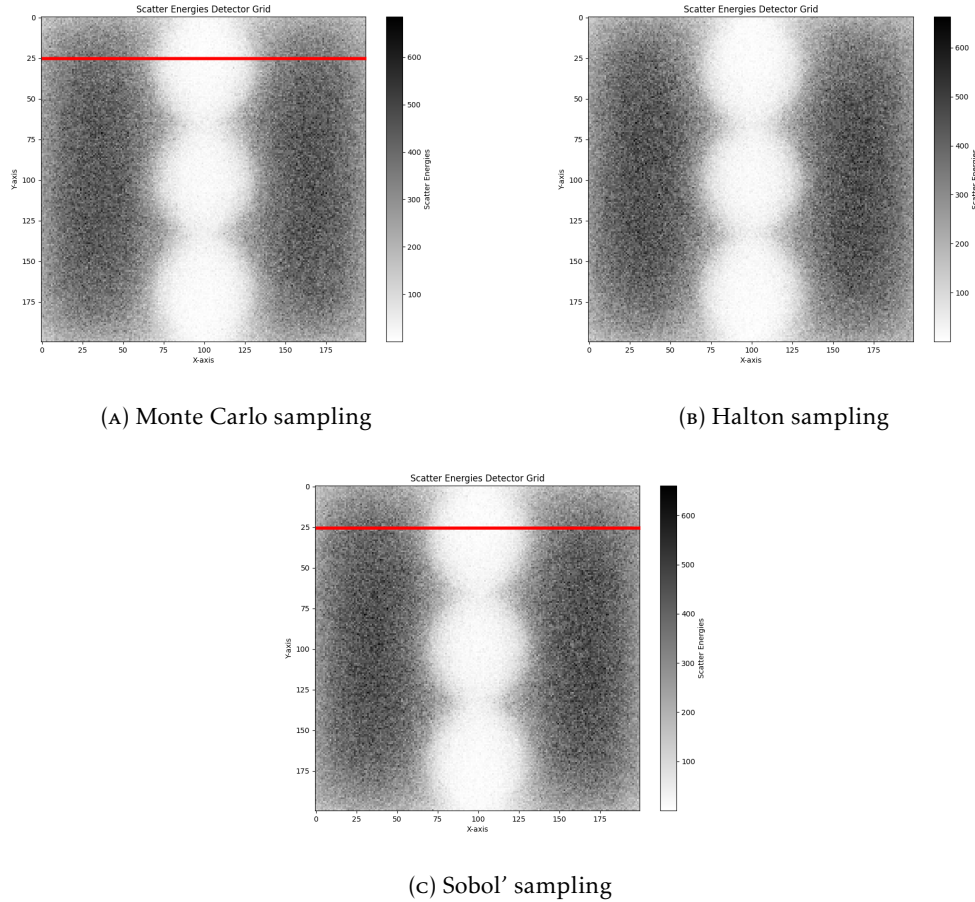
FIGURE 11.6: Simulated scatter intensities for an X-ray of the Bone-in-Water phantom using Monte Carlo, Halton and Sobol' sampling.
