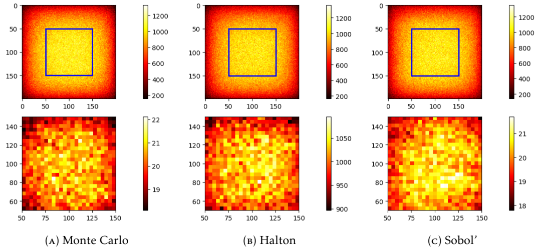
FIGURE 11.8: Comparison intensity grids of scattered photons for the Water-Wall phantom using different sampling strategies.
