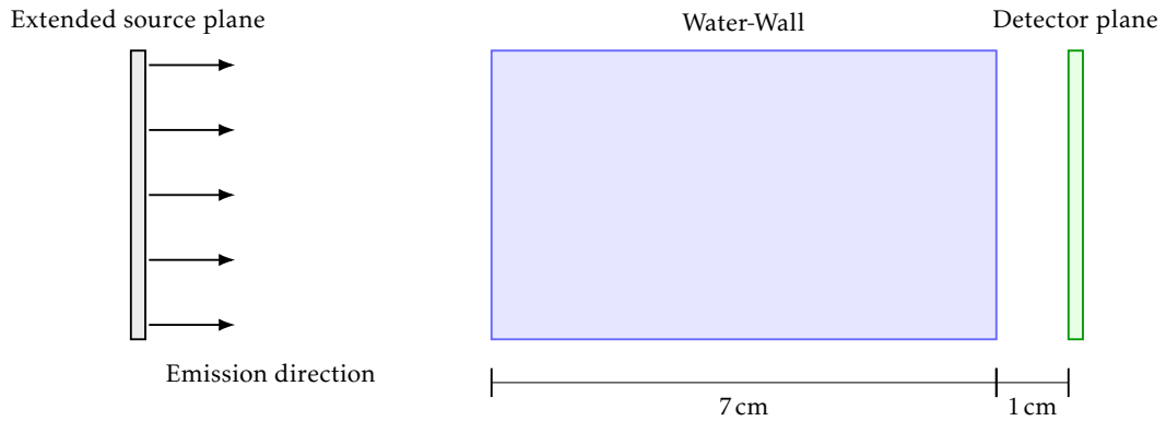
FIGURE 11.1: Schematic setup of the Water-Wall Scene.
