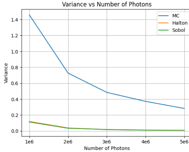
FIGURE 11.5: Plot of noise levels for primary intensities in Water-Wall Phantom for varying numbers of simulated photons.
