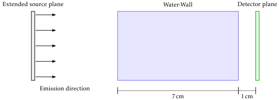
FIGURE 11.1: Schematic setup of the water-wall scene.
