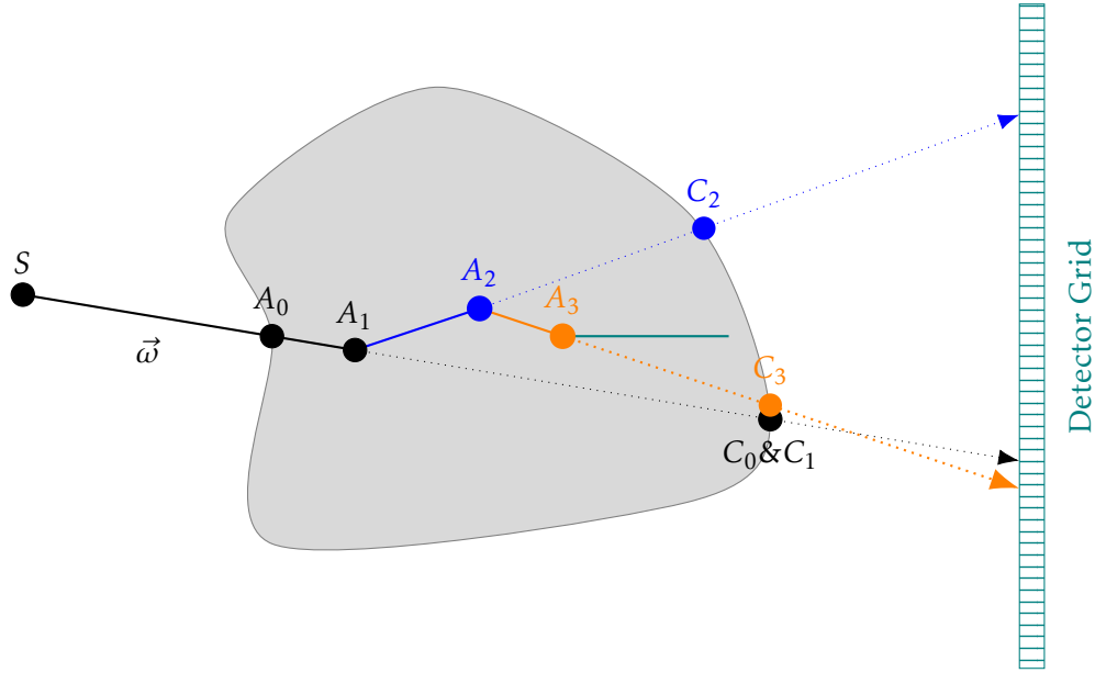
FIGURE 10.1: Illustration of the ray paths of a photon. The photon is emitted at the position S with direction \vec{w} and scattered at A_1 , A_2 and A_3 .
