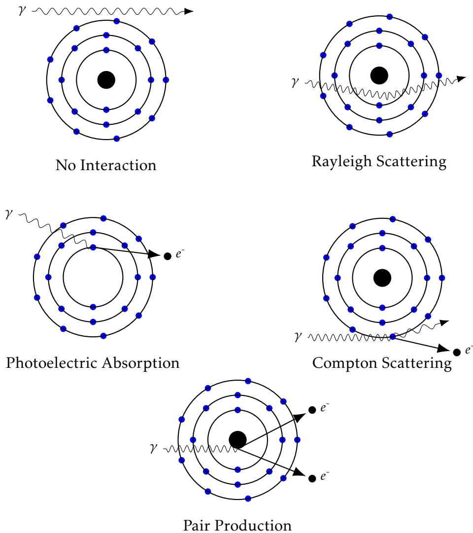
FIGURE 9.6: Principles from photon interaction with matter similar to [18, Chap. 7]
