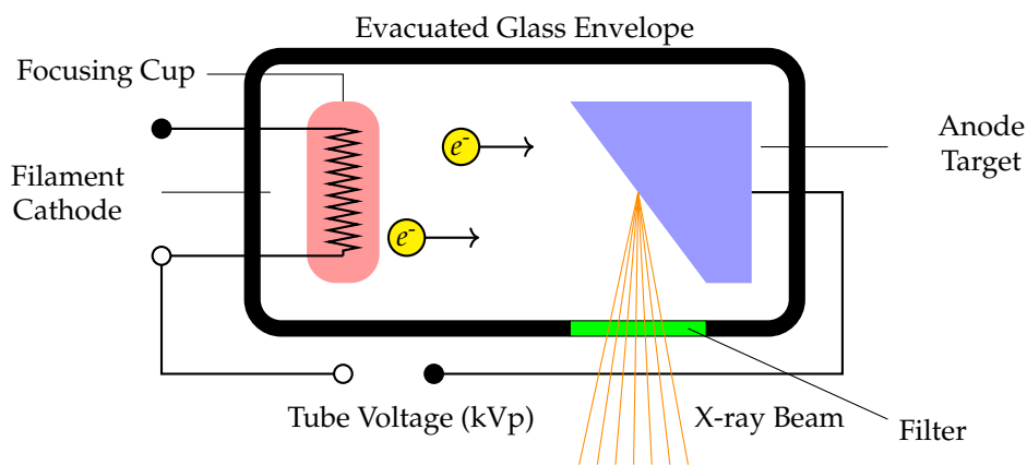
FIGURE 9.5: Schematic of an X-ray tube with Filter.
