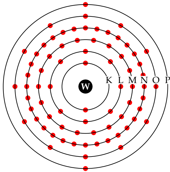
FIGURE 9.3: Bohr model of the tungsten atom (W, Z = 74 ) with electron shells and subshells.
