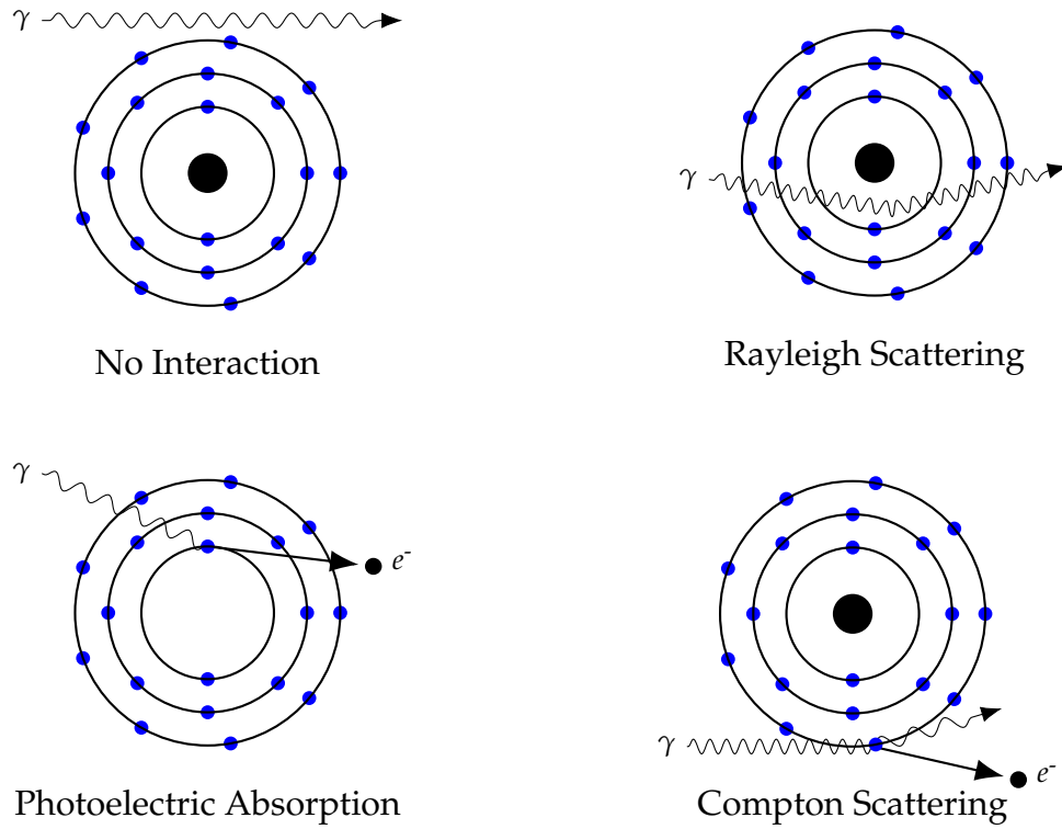
FIGURE 9.7: Principles from photon interaction with matter similar to [13, Chap. 7]
