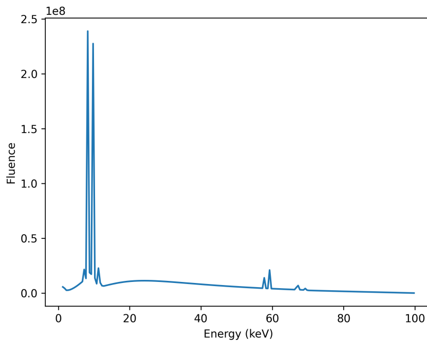
FIGURE 9.4: X-ray spectrum for a tungsten cathode at 100 kVp showing the continuous bremsstrahlung spectrum and characteristic peaks. Build with SpekPy [19]
