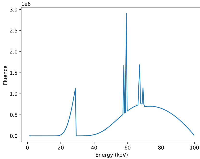
FIGURE 9.6: X-ray spectrum for a tungsten cathode at 100 kVp with a 0.4 mm showing the continuous bremsstrahlung spectrum and characteristic peaks. Build with SpekPy [19]
