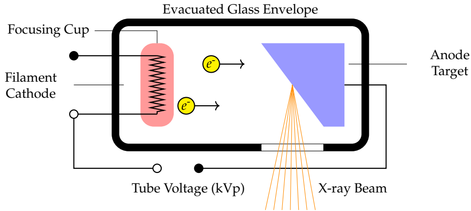
FIGURE 9.2: Schematic of an X-ray tube.
