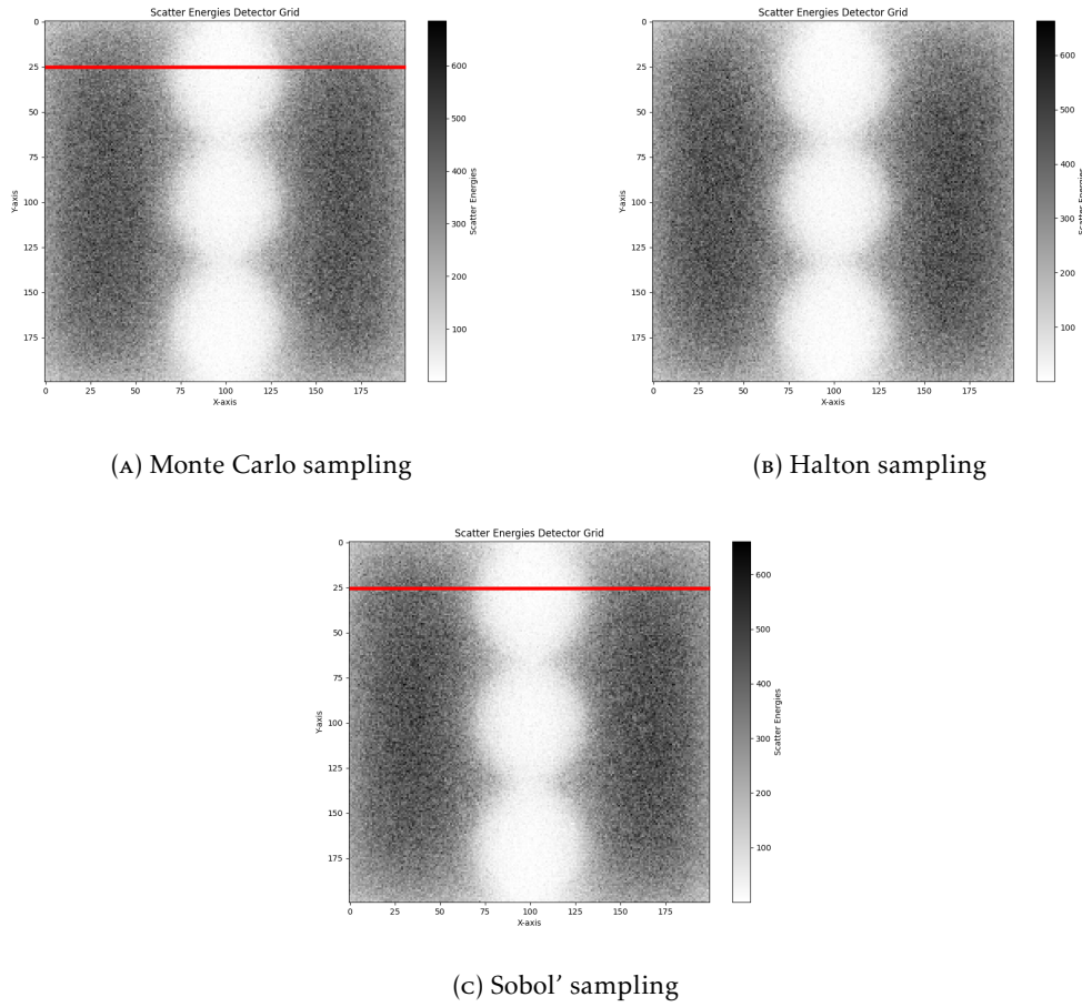
FIGURE 12.6: Simulated scatter intensities for an X-ray of the bone-in-water phantom using Monte Carlo, Halton and Sobol' sampling.
