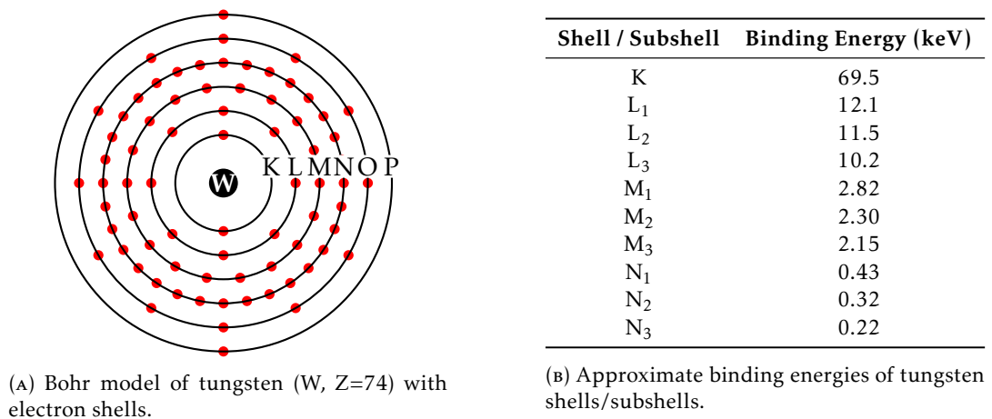
FIGURE 10.3: (a) Tungsten atom schematic and (b) corresponding binding energies.
