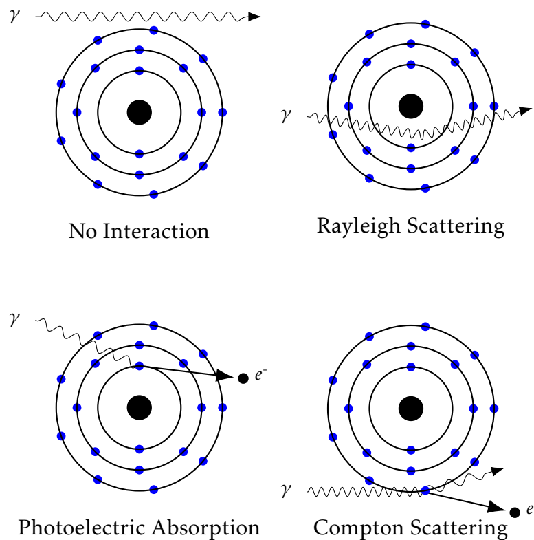
FIGURE 10.6: Principles from photon interaction with matter similar to [20, Chap. 7]
