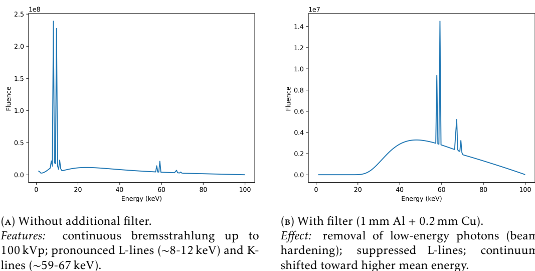
FIGURE 10.4: X-ray spectra for a tungsten anode at 100 kVp: (a) without and (b) with added filtration. The filter selectively attenuates low-energy photons, reducing patient dose while preserving higher-energy components. Both spectra were generated using SpekPy [28].
