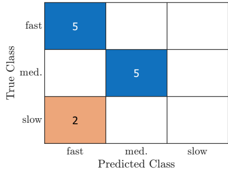
c) Conf. matrix PO model + SIM
