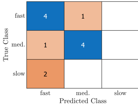
b) Confusion matrix PO model
