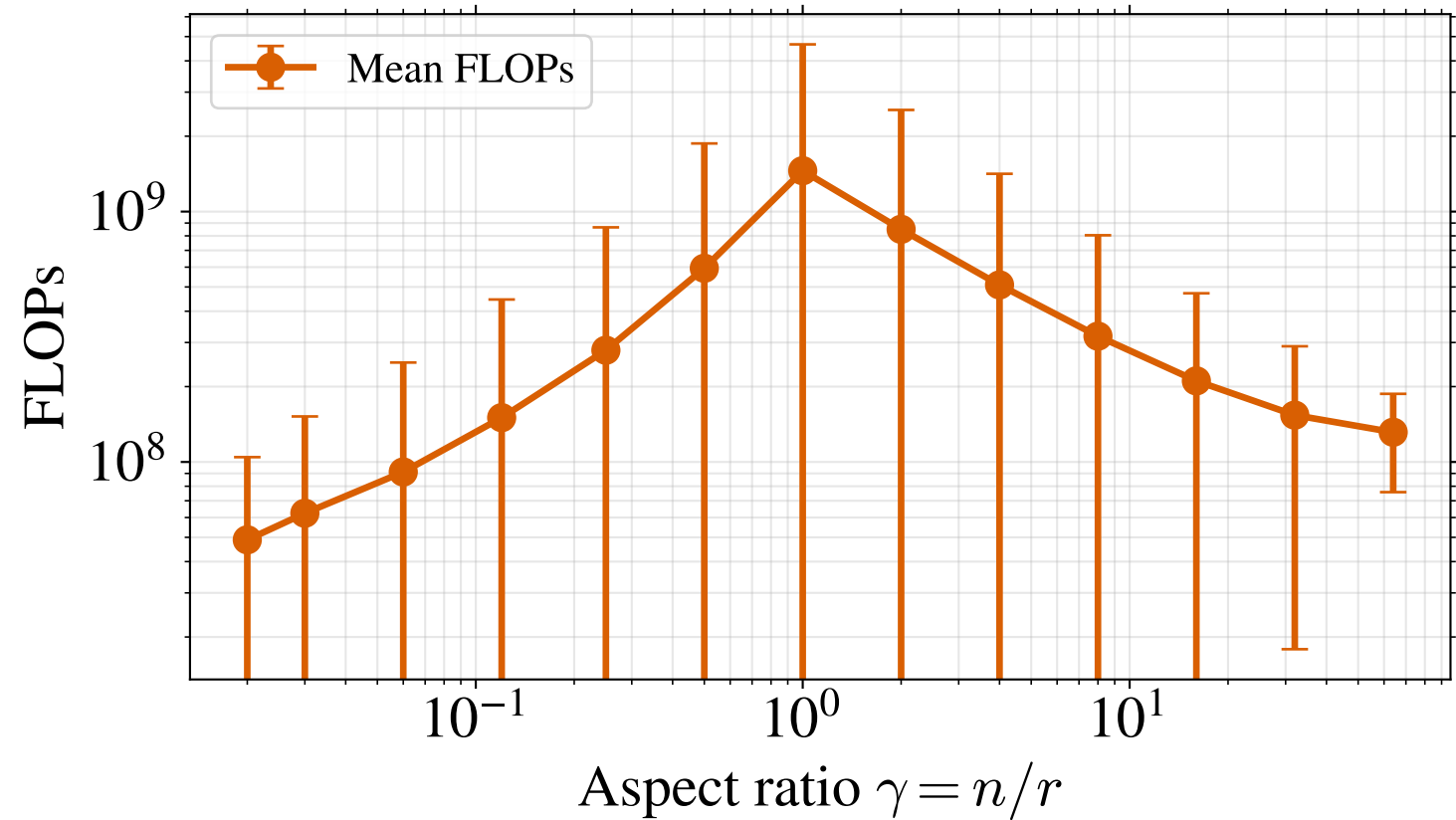
FLOPs vs Aspect Ratio \gamma
