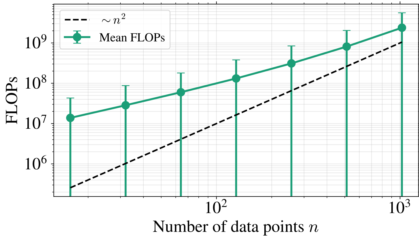
FLOPs vs Data Size: \sim n^2
