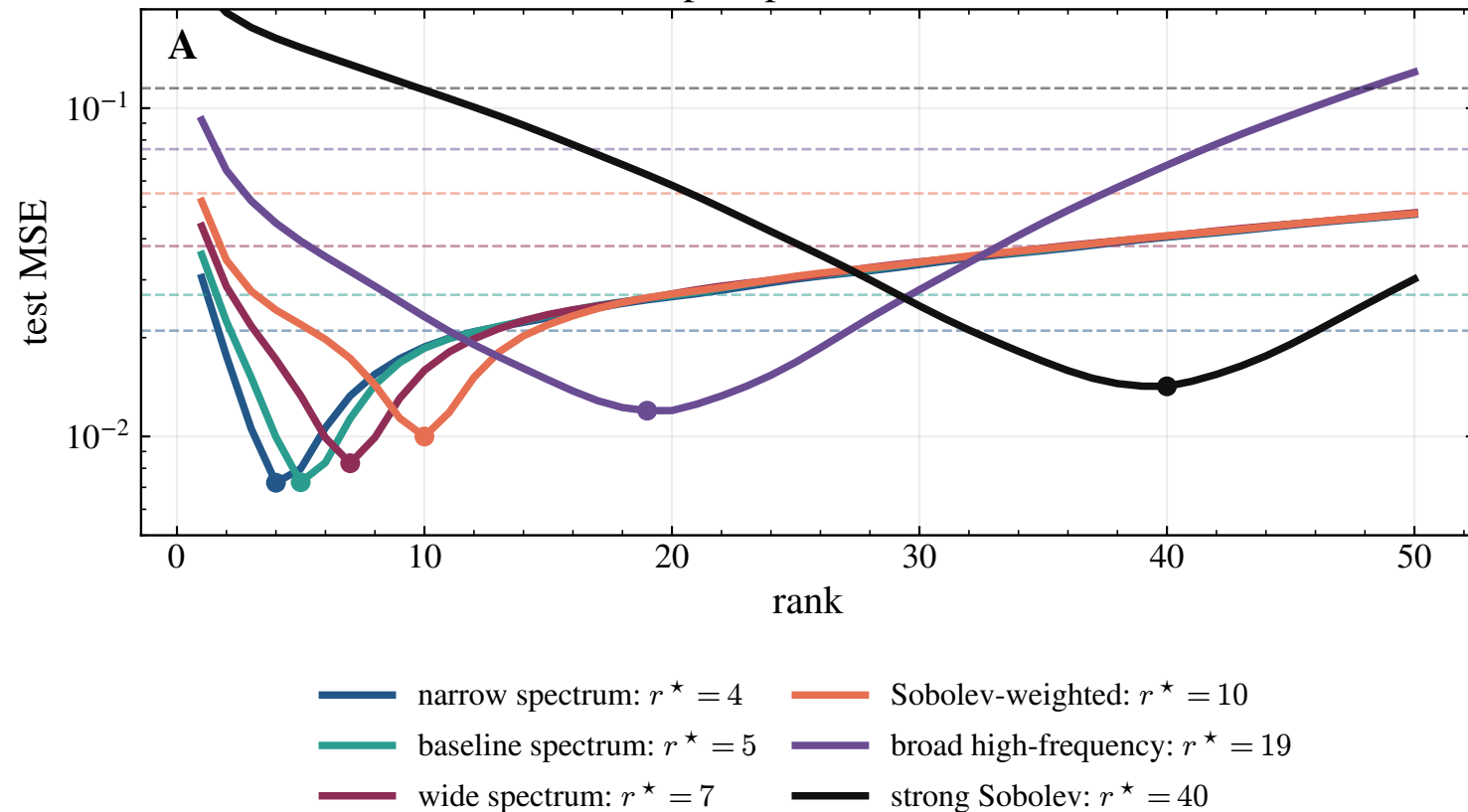
Control sweeps: optimum rank can move
