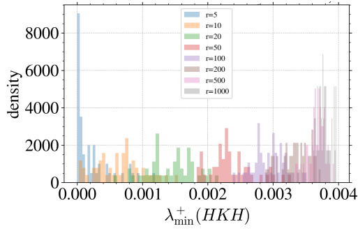
Figure 8: * Histograms of \lambda_{\min}^+(HKH) ; matrix stays PSD.
