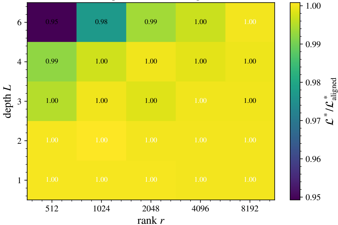
Rank and depth bend the scaling-law floor
