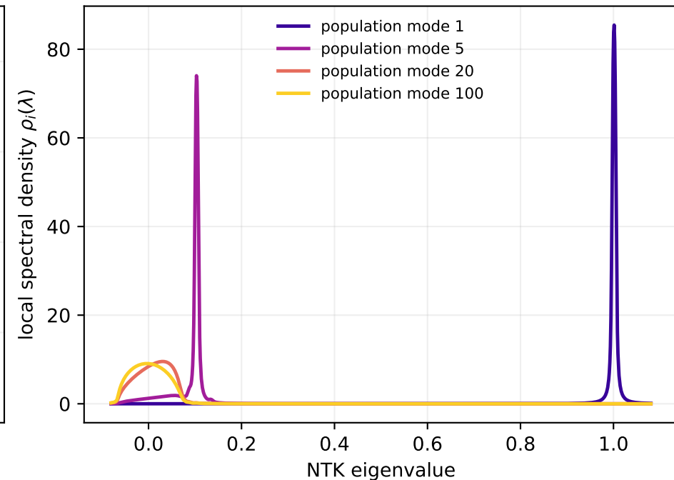
eigenvector mixing, mode by mode
