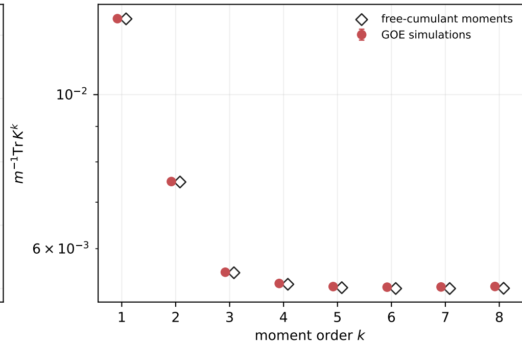
independent moment check
