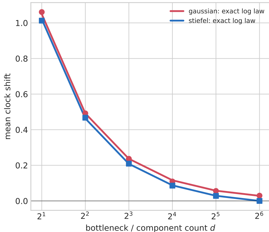
Wishart vs. Weingarten clock
