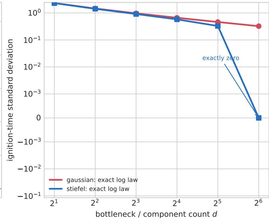
Full-rank Stiefel cancellation
