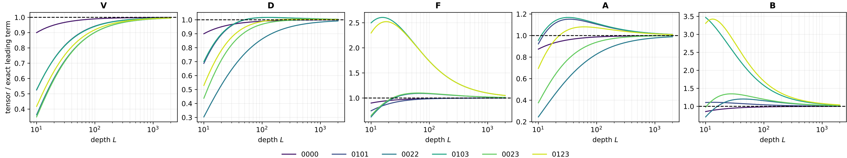
Convergence to the componentwise critical ReLU coefficients
