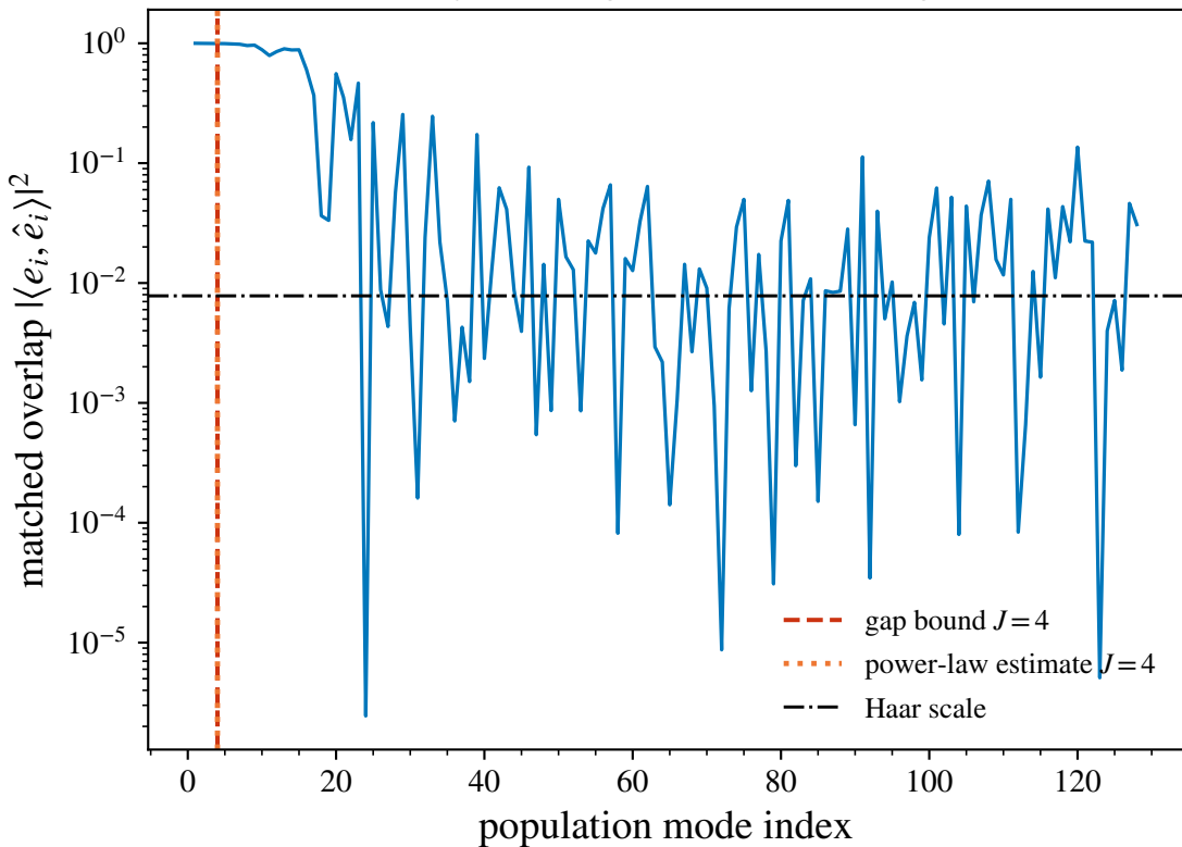
Head stability and Wigner-like tail mixing, \tau=0.02
