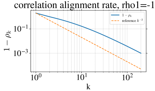
Figure 3: Correlation alignment along depth: 1 - \rho_k = O(k^{-2}) (log-log) as in Theorem 5.
