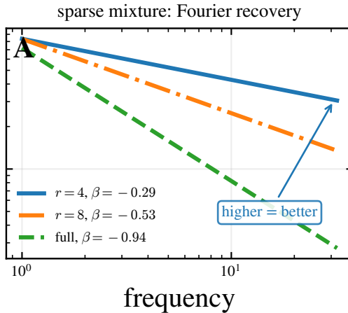
normalized excess MSE
